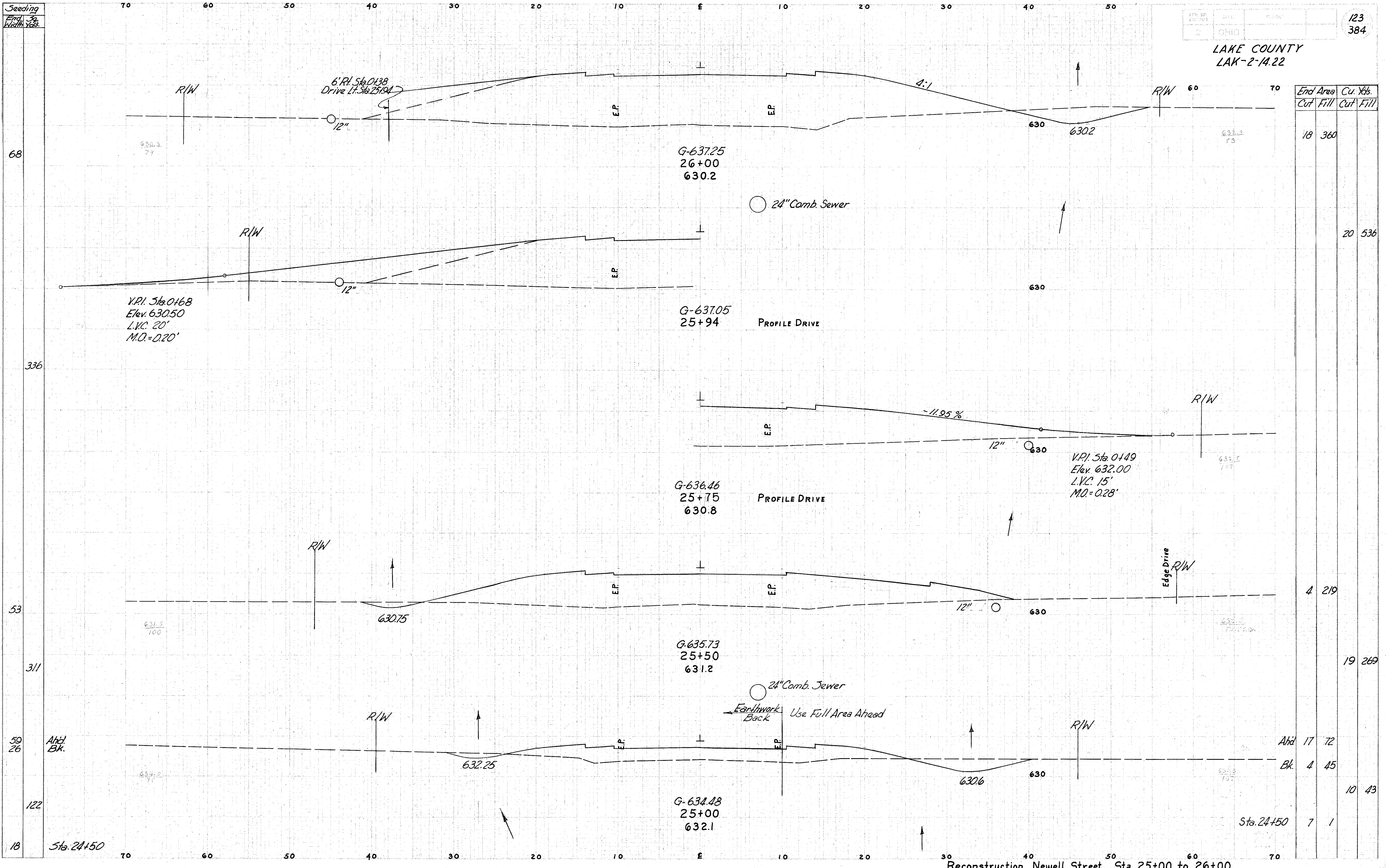
Reconstruction Newell Street Sta. 25+00 to 26+00
