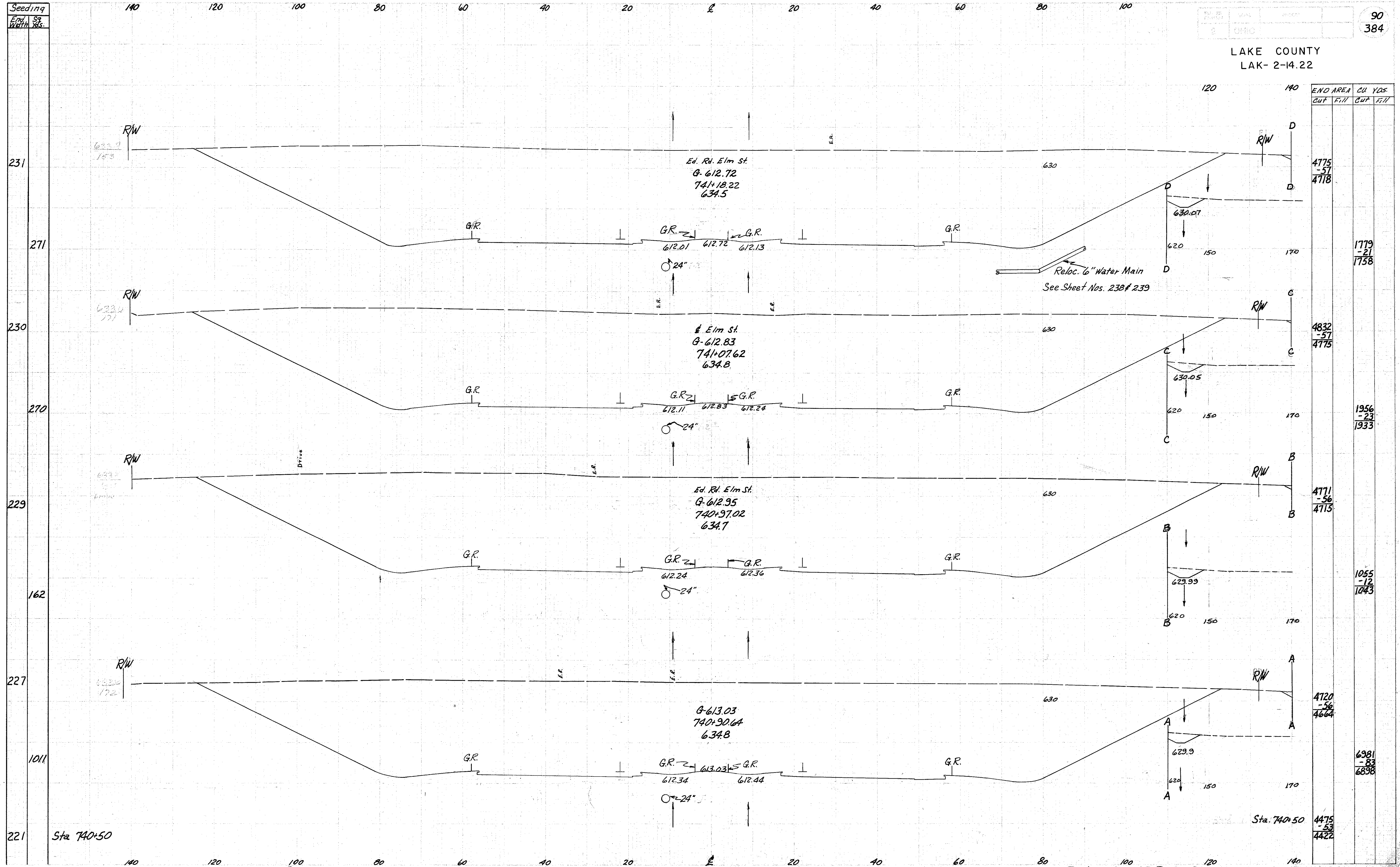
Relocation S.R. 2 Sta. 740+90.64 to 741+18.22
