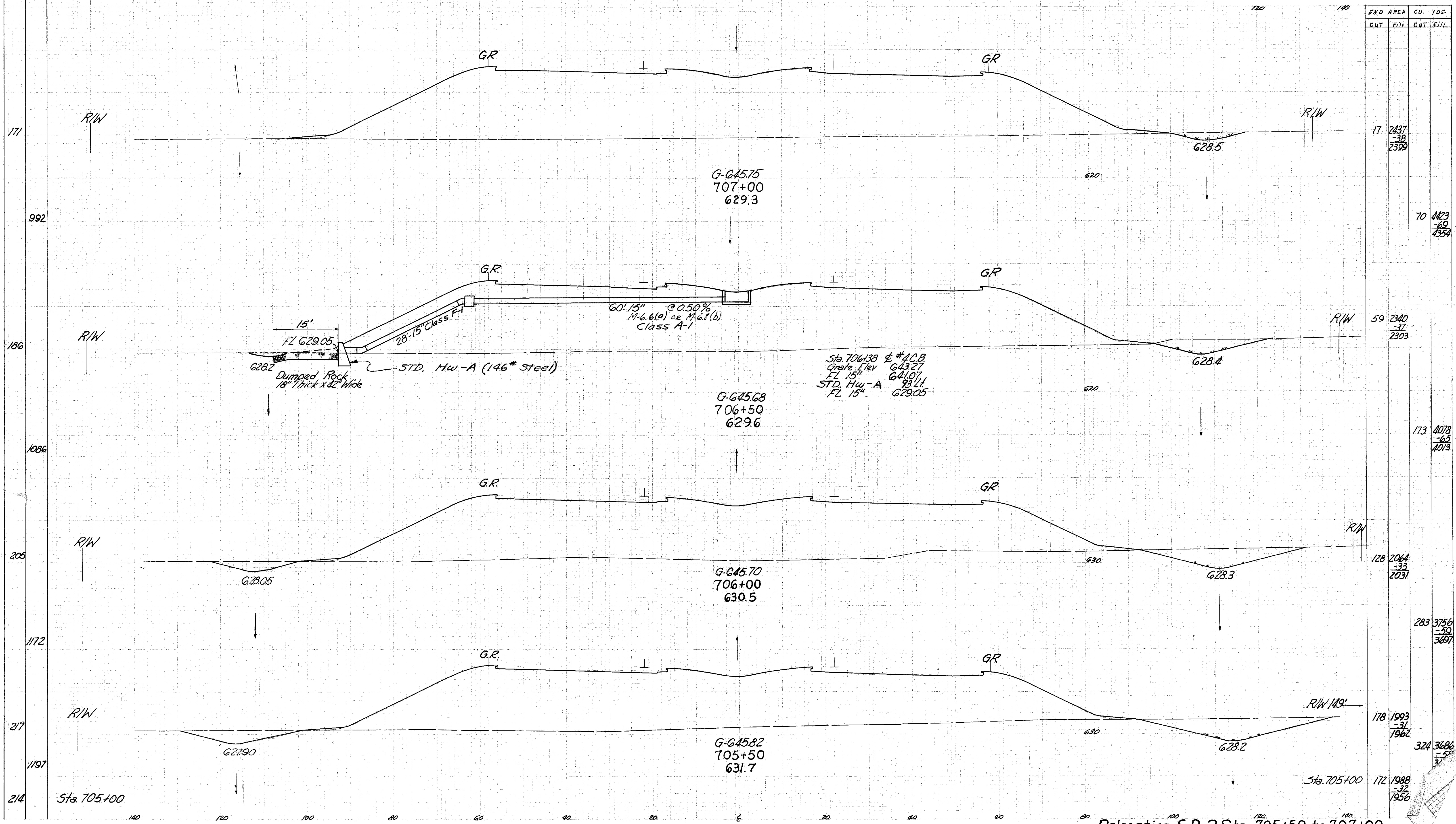
Relocation S.R.2 Sta. 705+50 to 707+00
