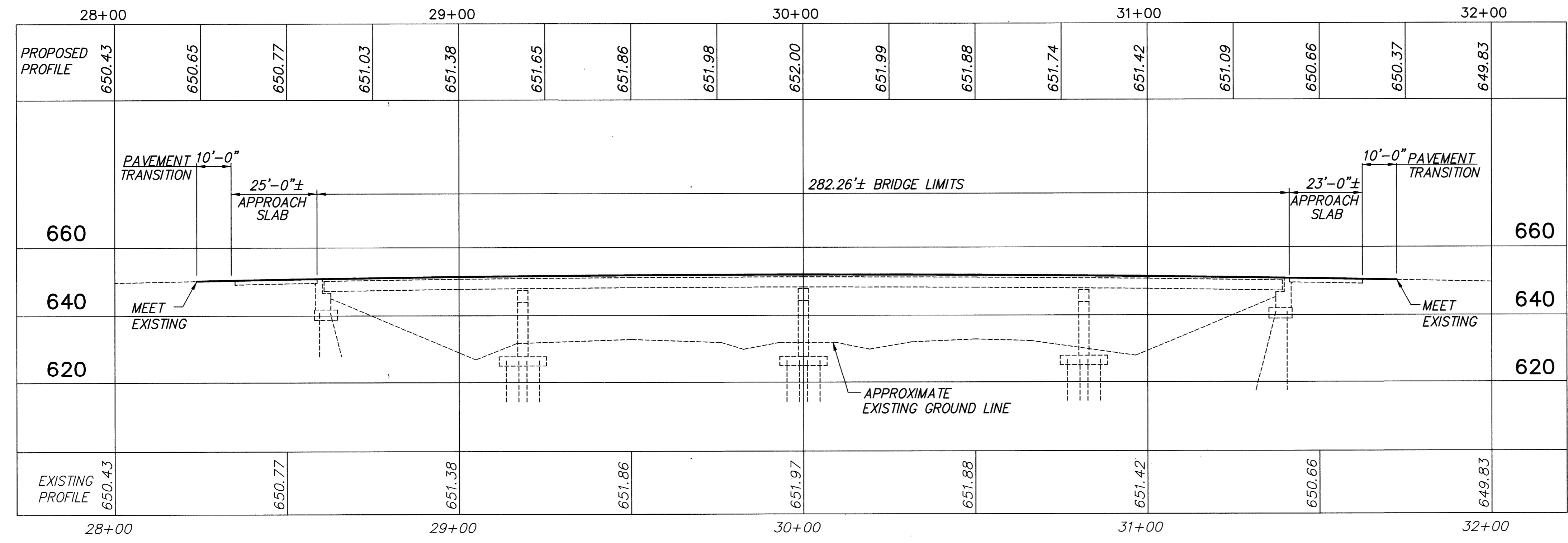
PROFILE ALONG \bar{C} SURVEY
