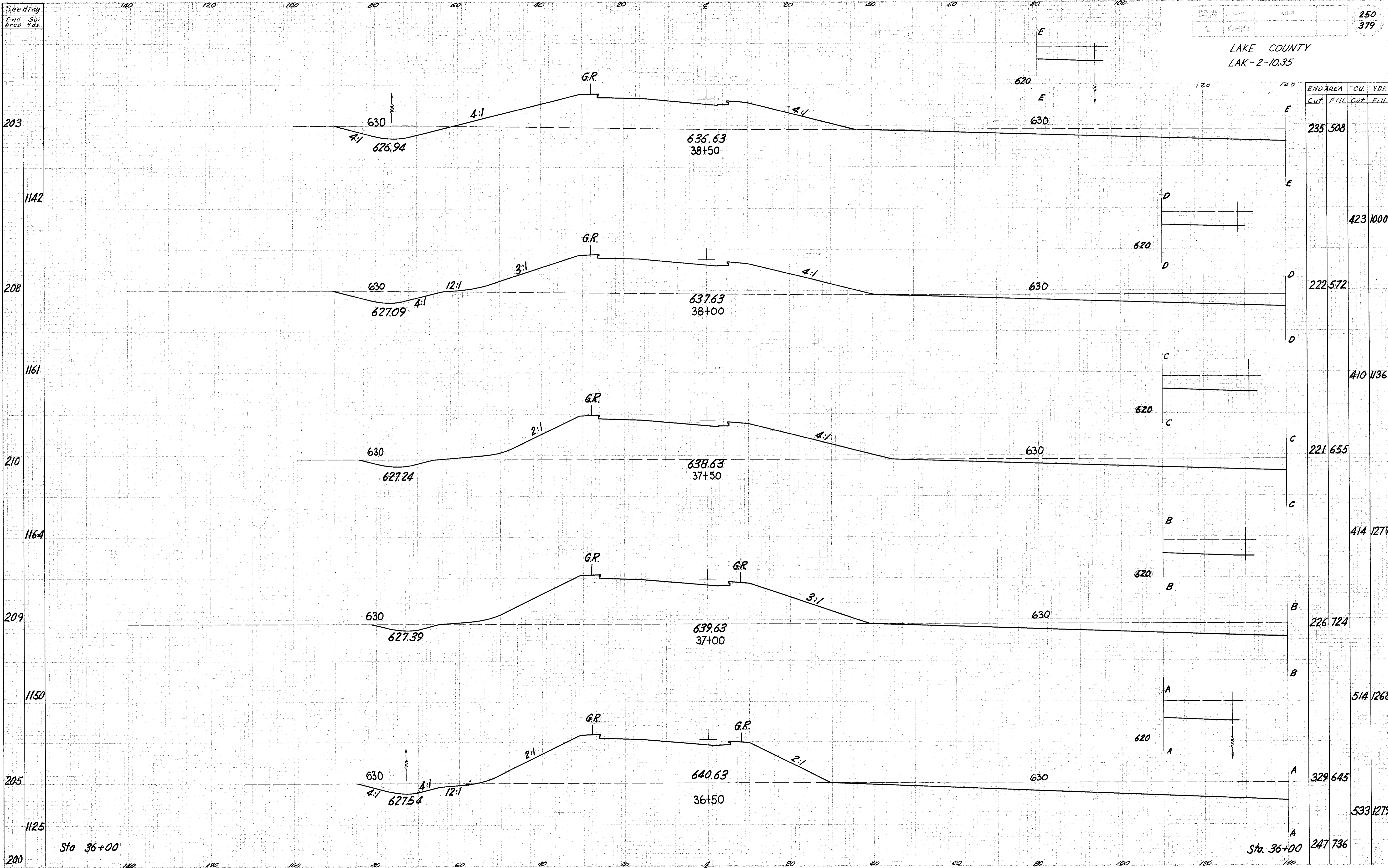
Ramp "G" Sta. 36+50 to 38+50
