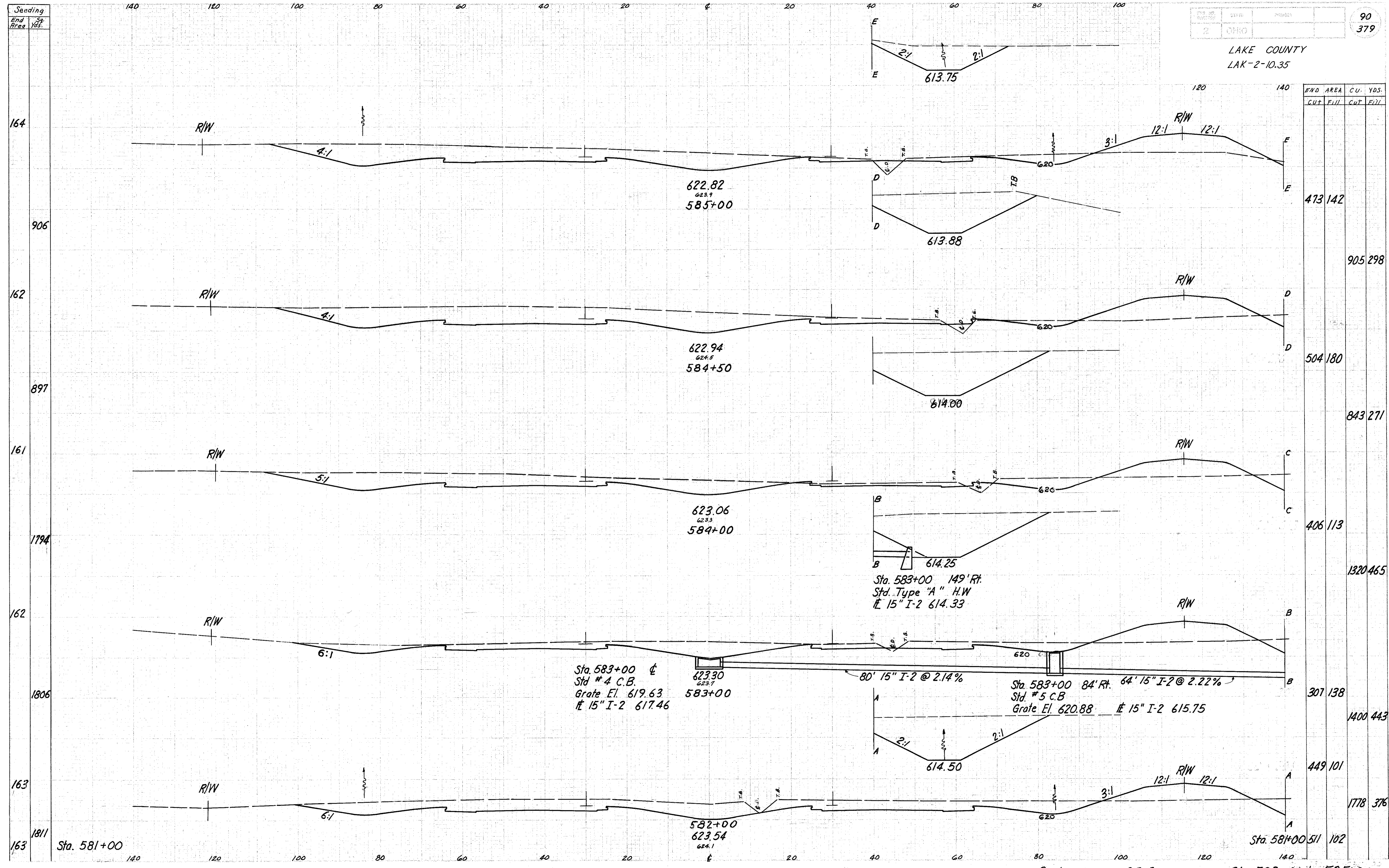
Relocation SR 2 Sta. 582+00 to 585+00
