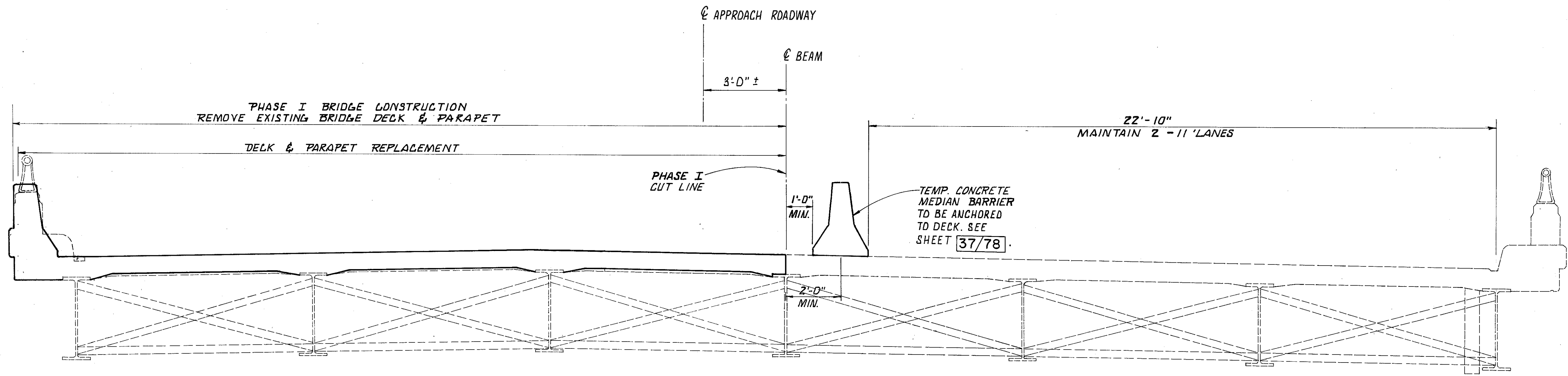
PHASE I (LOOKING EAST) LAK-2-0363 R AS SHOWN LAK-2-0363 L OPPOSITE HAND
