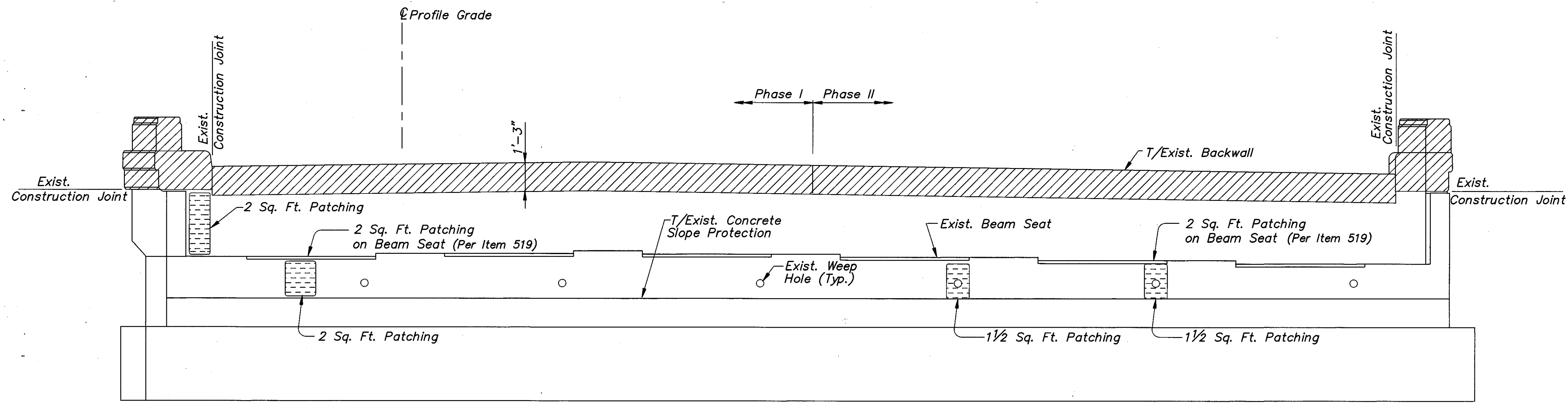
ELEVATION REAR ABUTMENT
