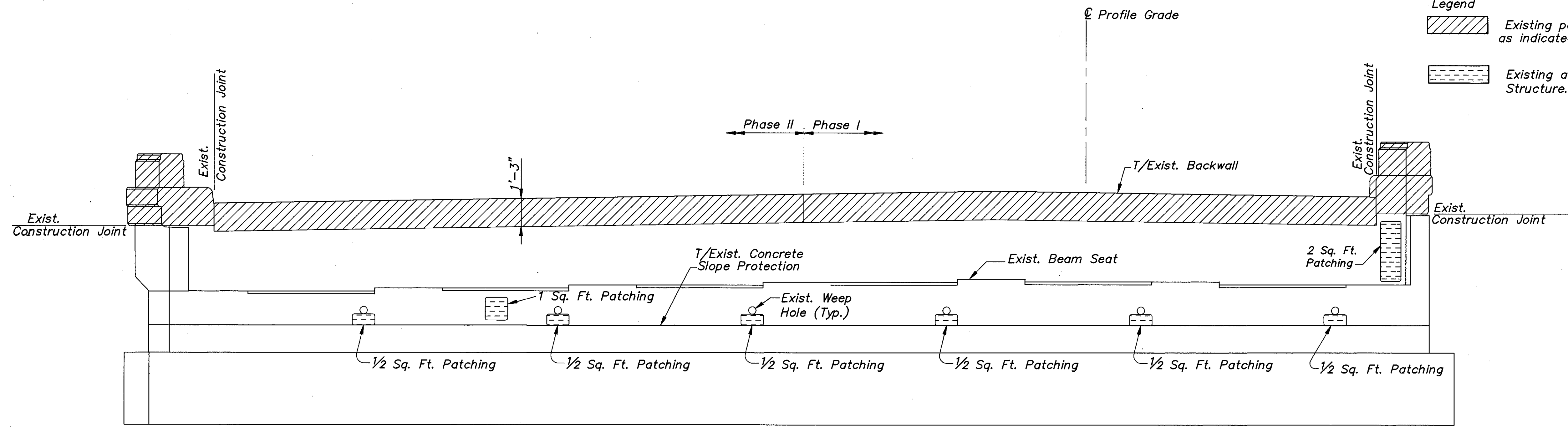
ELEVATION FORWARD ABUTMENT
