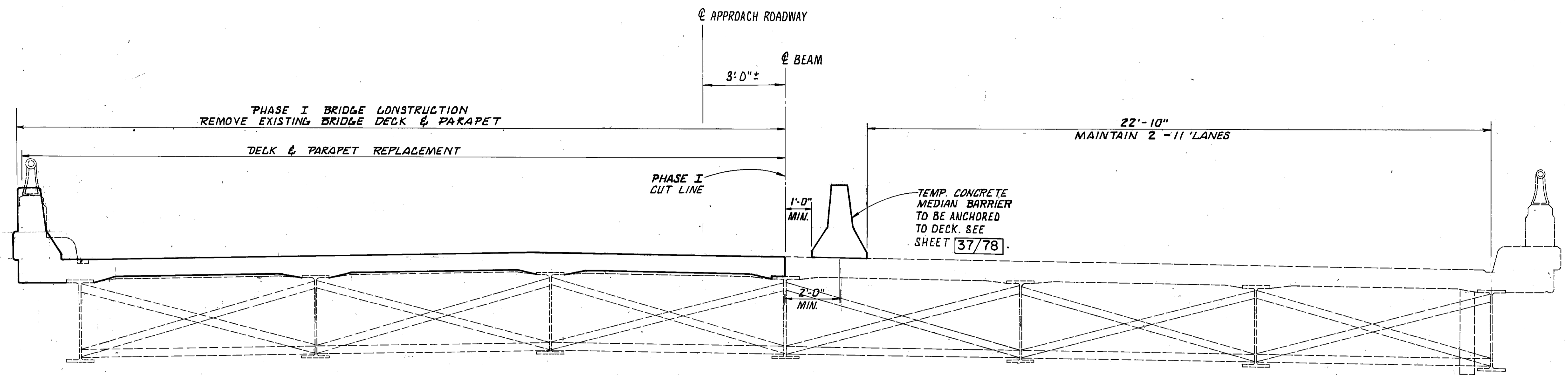
PHASE I (LOOKING EAST) LAK-2-0180 R AS SHOWN LAK-2-0180 L OPPOSITE HAND
