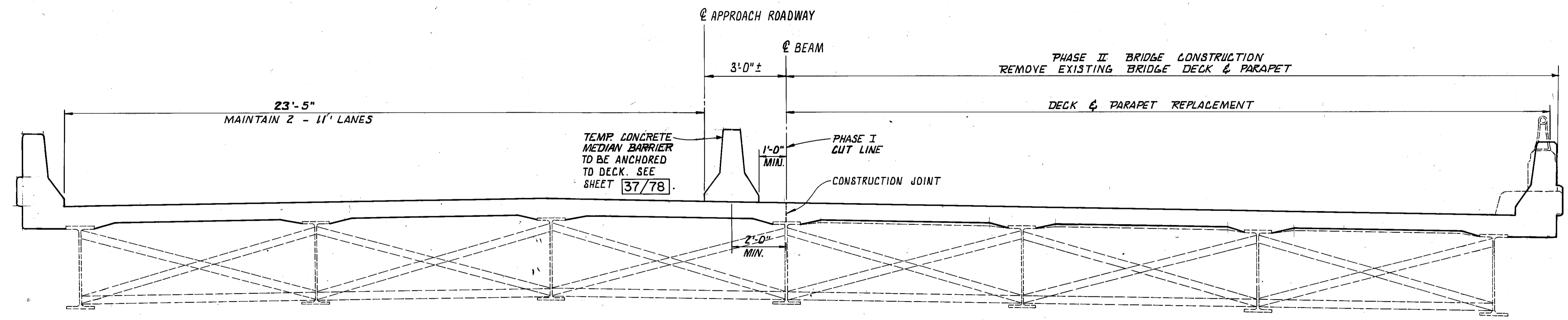
PHASE II (LOOKING EAST) LAK-2-0180 R AS SHOWN LAK-2-0180 L OPPOSITE HAND
