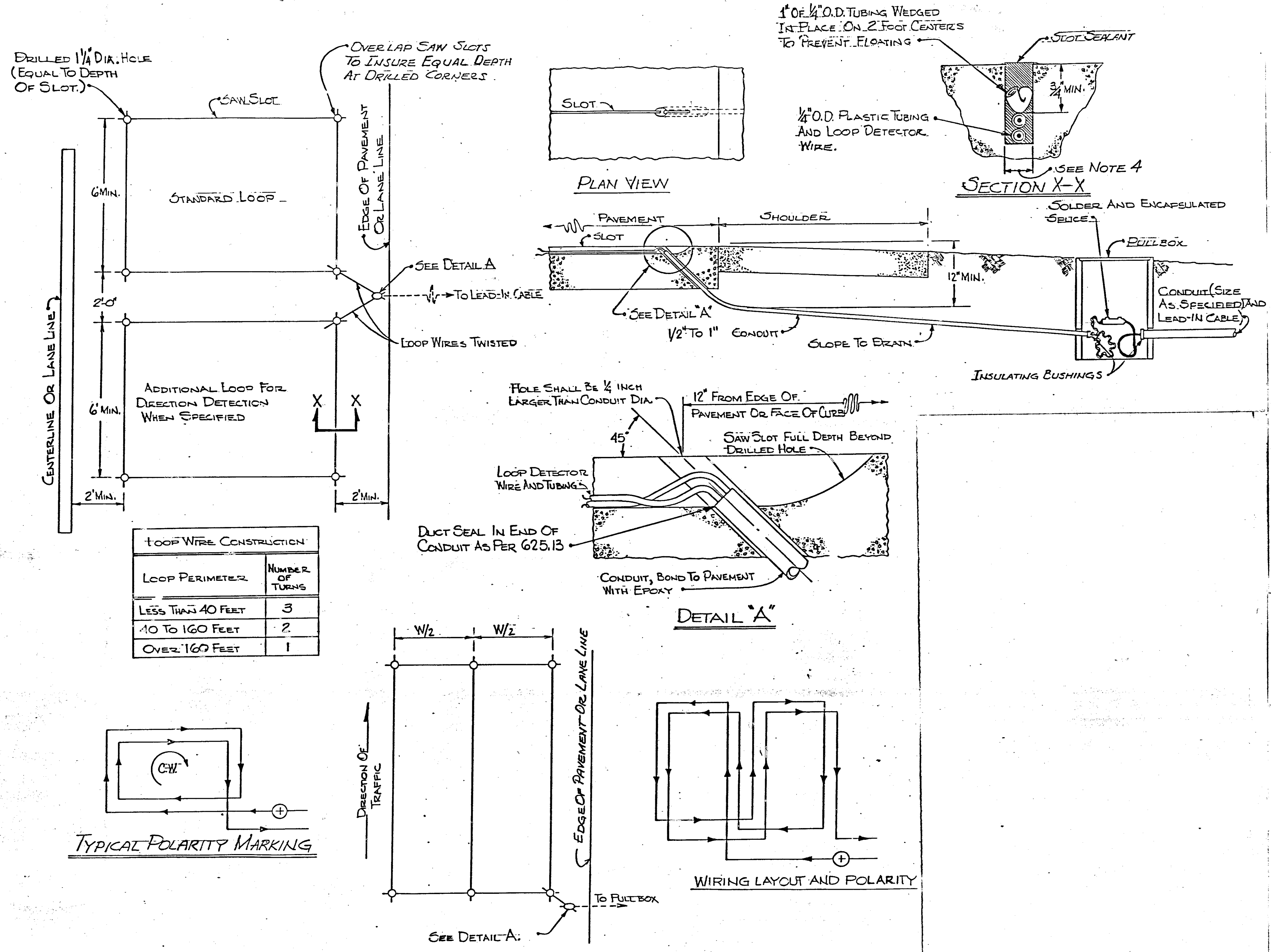
FIGURE 8 LOOP DETAILS
