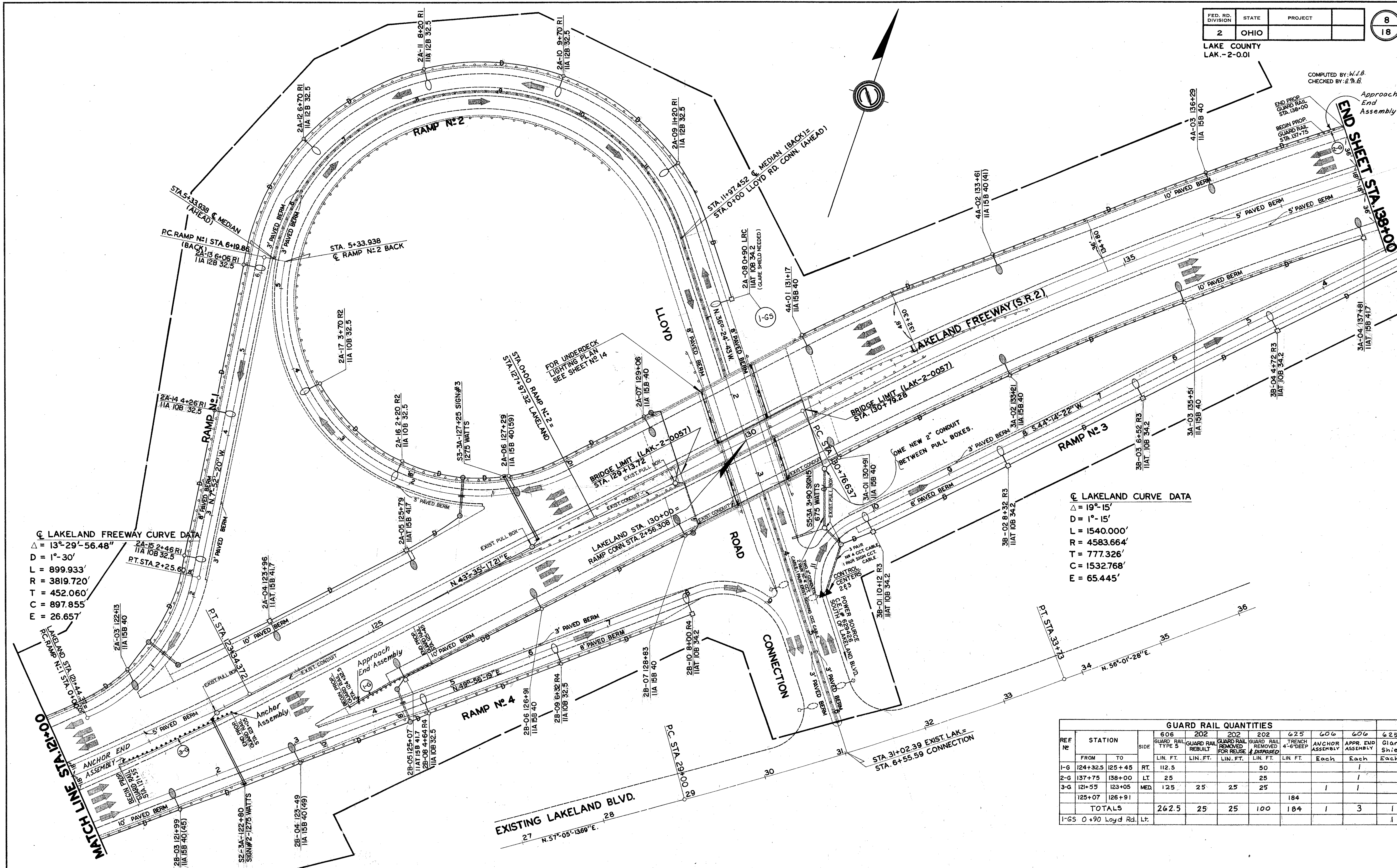
LIGHTING PLANS...LAKELAND FREEWAY (S.R.2) @ LLOYD RD. INTERCHANGE STA. 121+00 TO STA. 138+00
