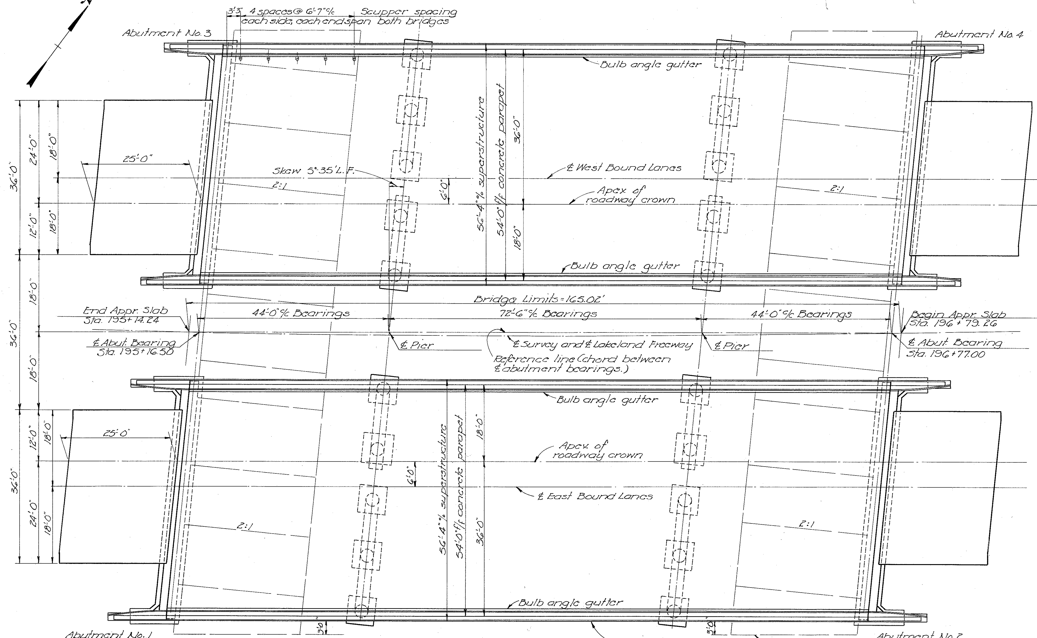
GENERAL PLAN
