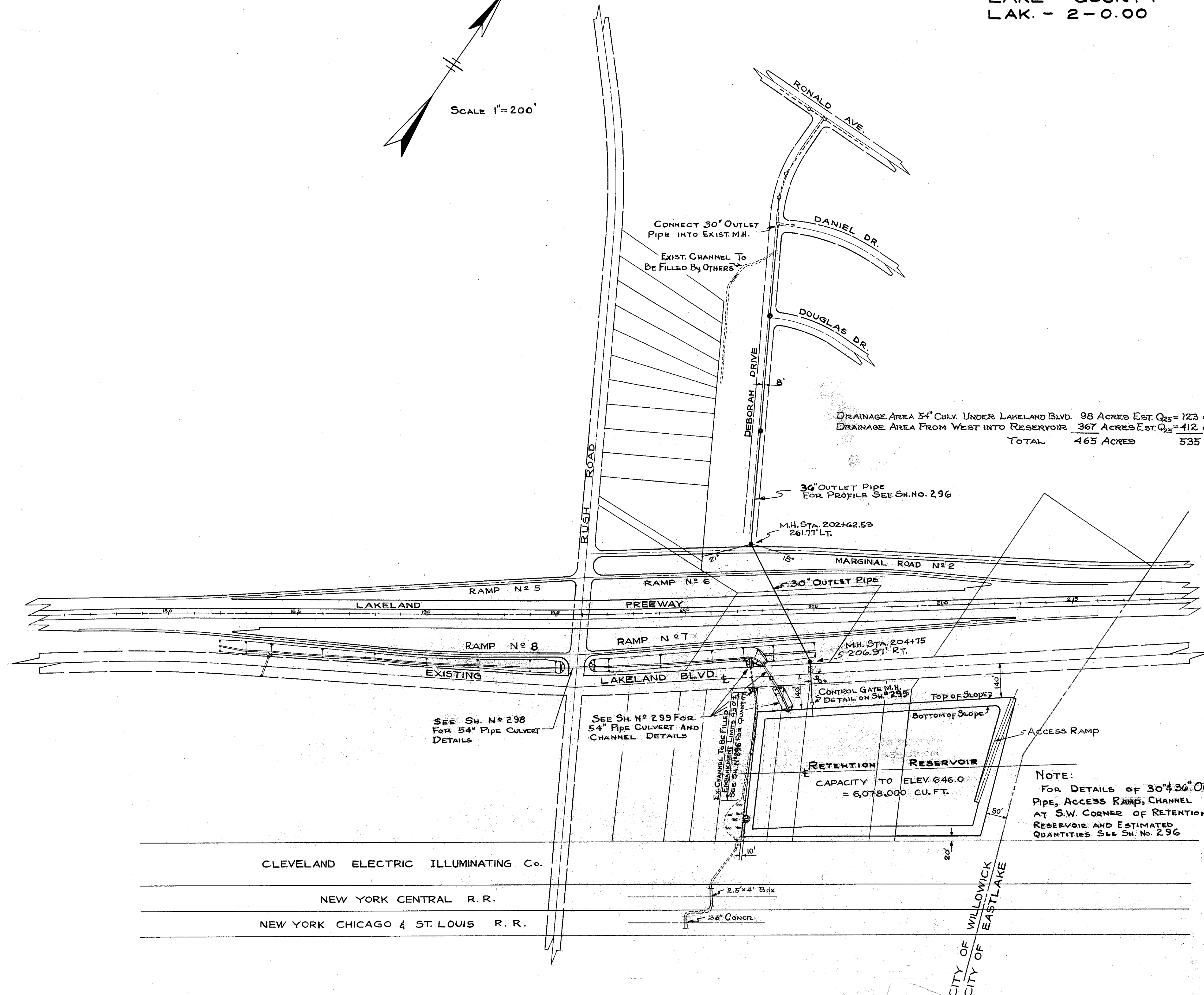
LOCATION PLAN - RETENTION RESERVOIR
