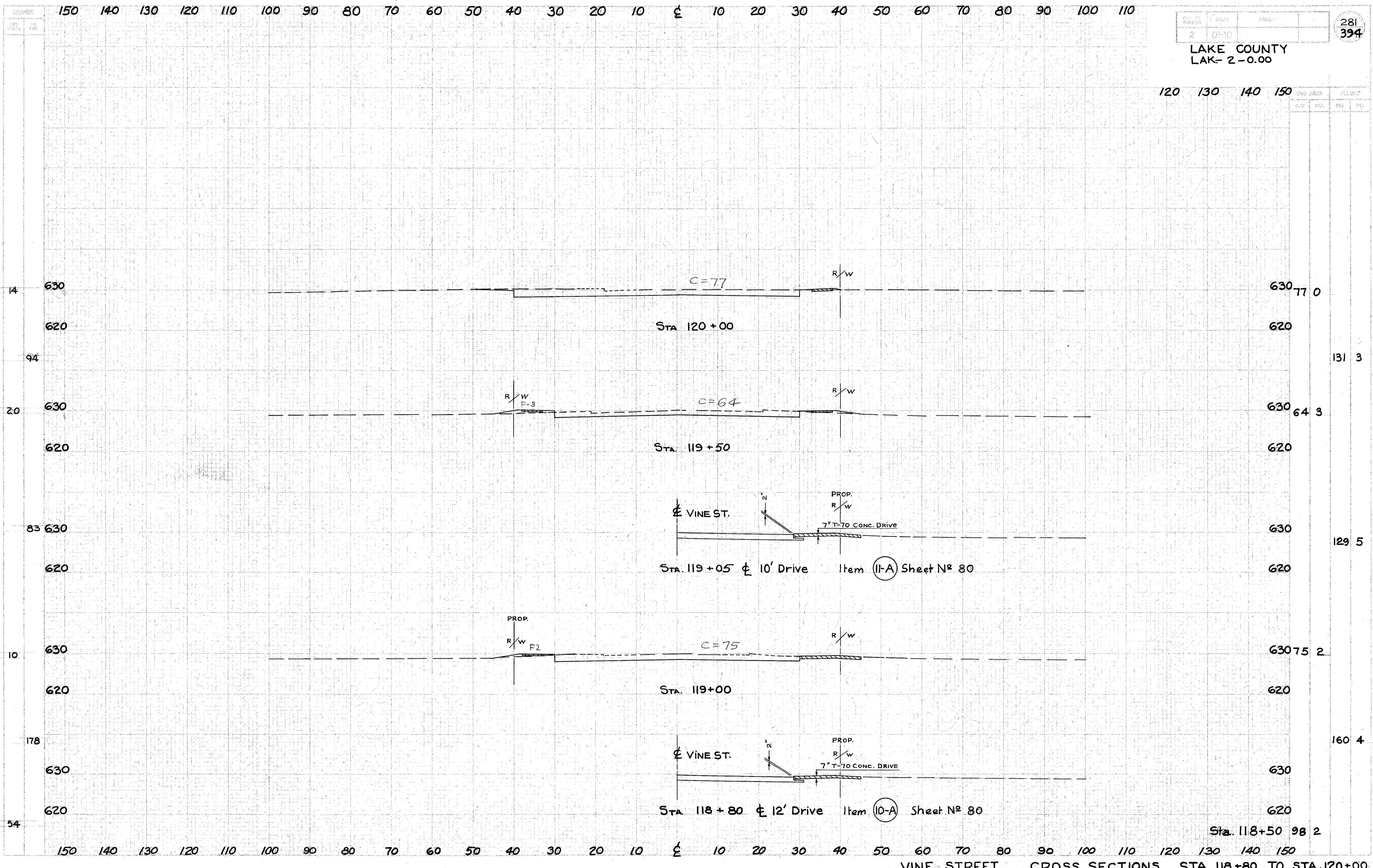
VINE STREET CROSS SECTIONS STA. 118+50 TO STA. 120+00
