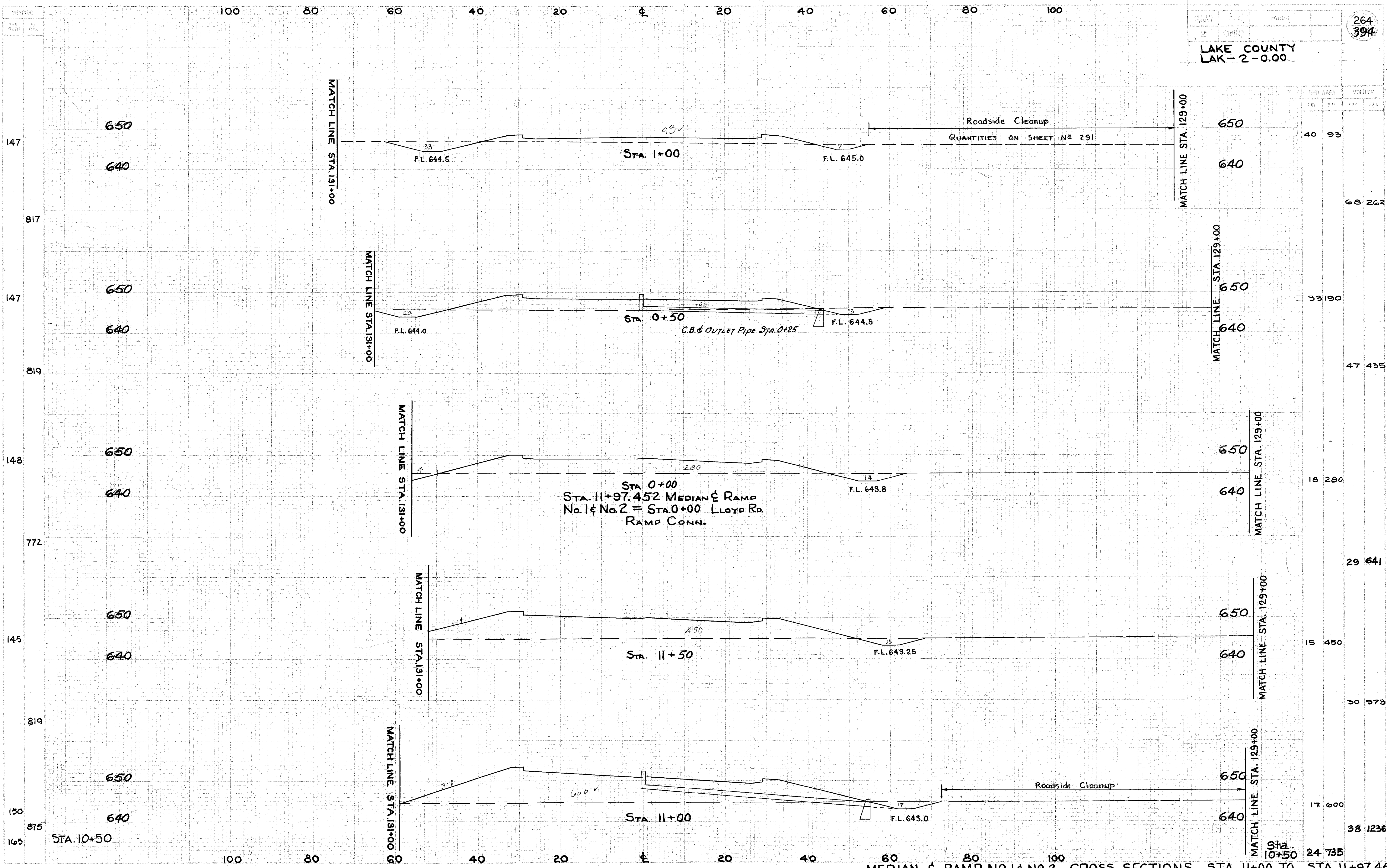
MEDIAN & RAMP NO 1 & NO 2 CROSS SECTIONS STA 11+00 TO STA 11+97.452 LLOYD RD. CONNECTION CROSS SECTIONS STA. 0+00 TO STA. 1+00
