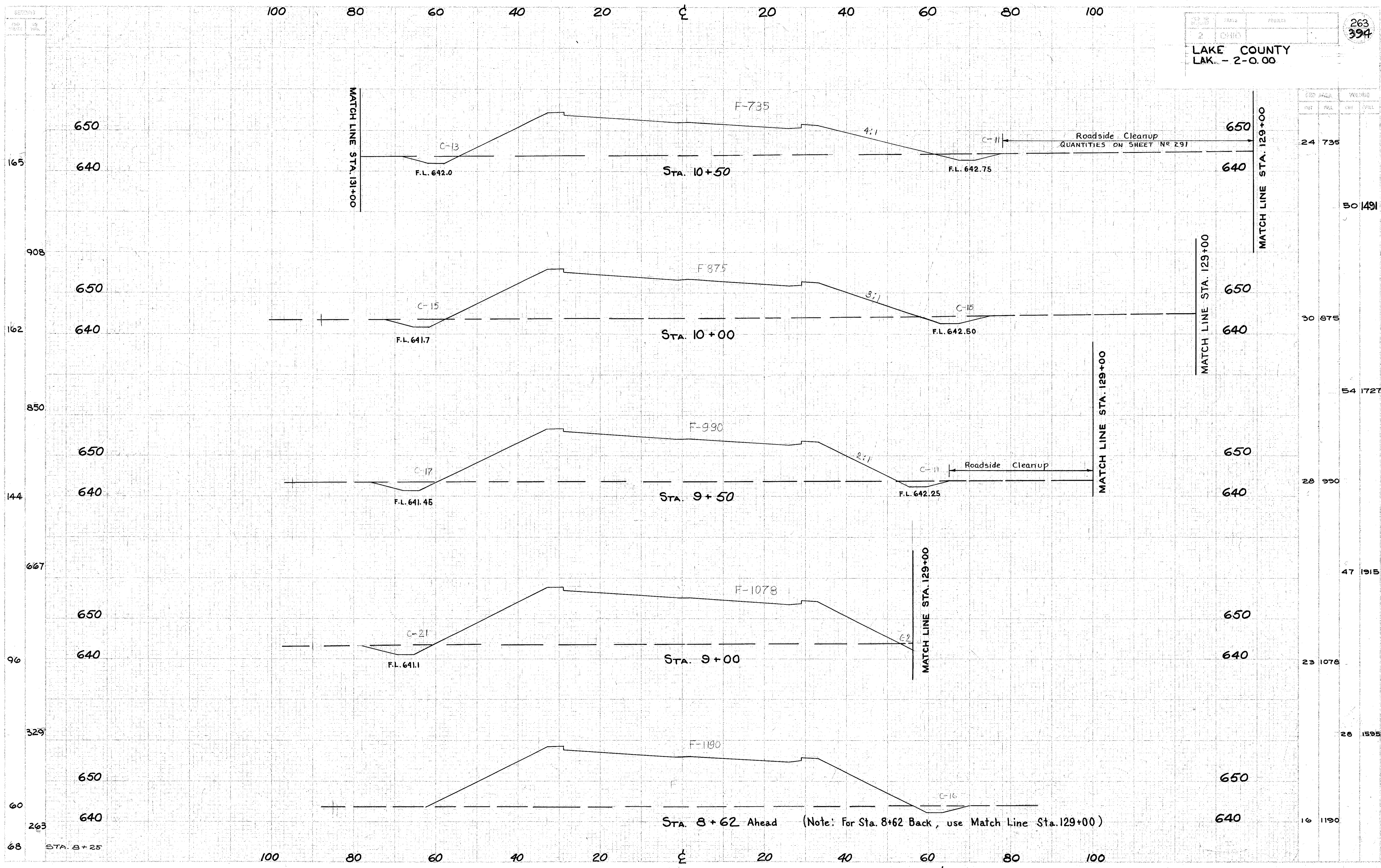
MEDIAN & RAMP #1 & RAMP #2 CROSS SECTIONS STA. 8+62 TO STA. 10+50
