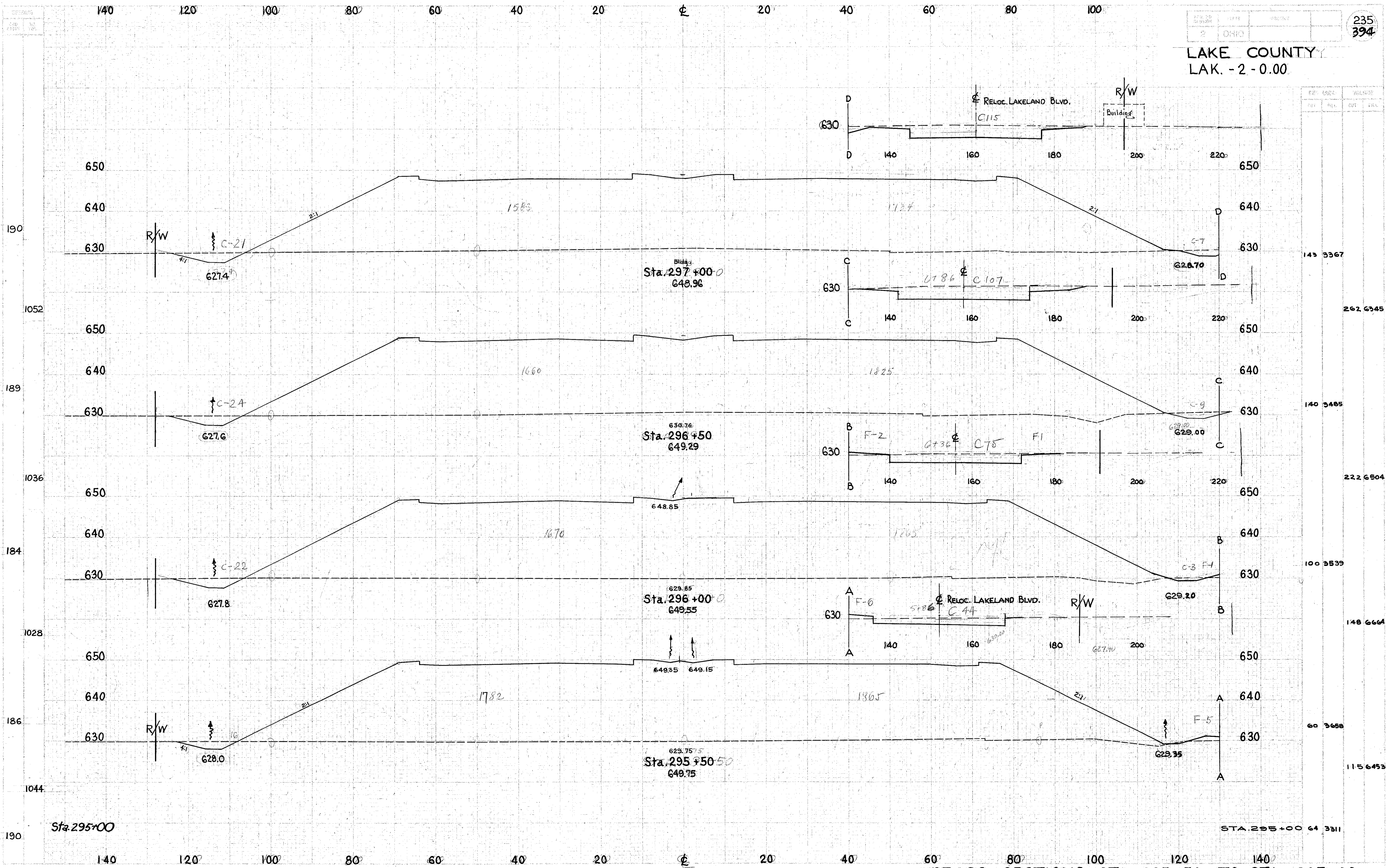
CROSS SECTIONS STA. 295+50 TO STA. 297+00
