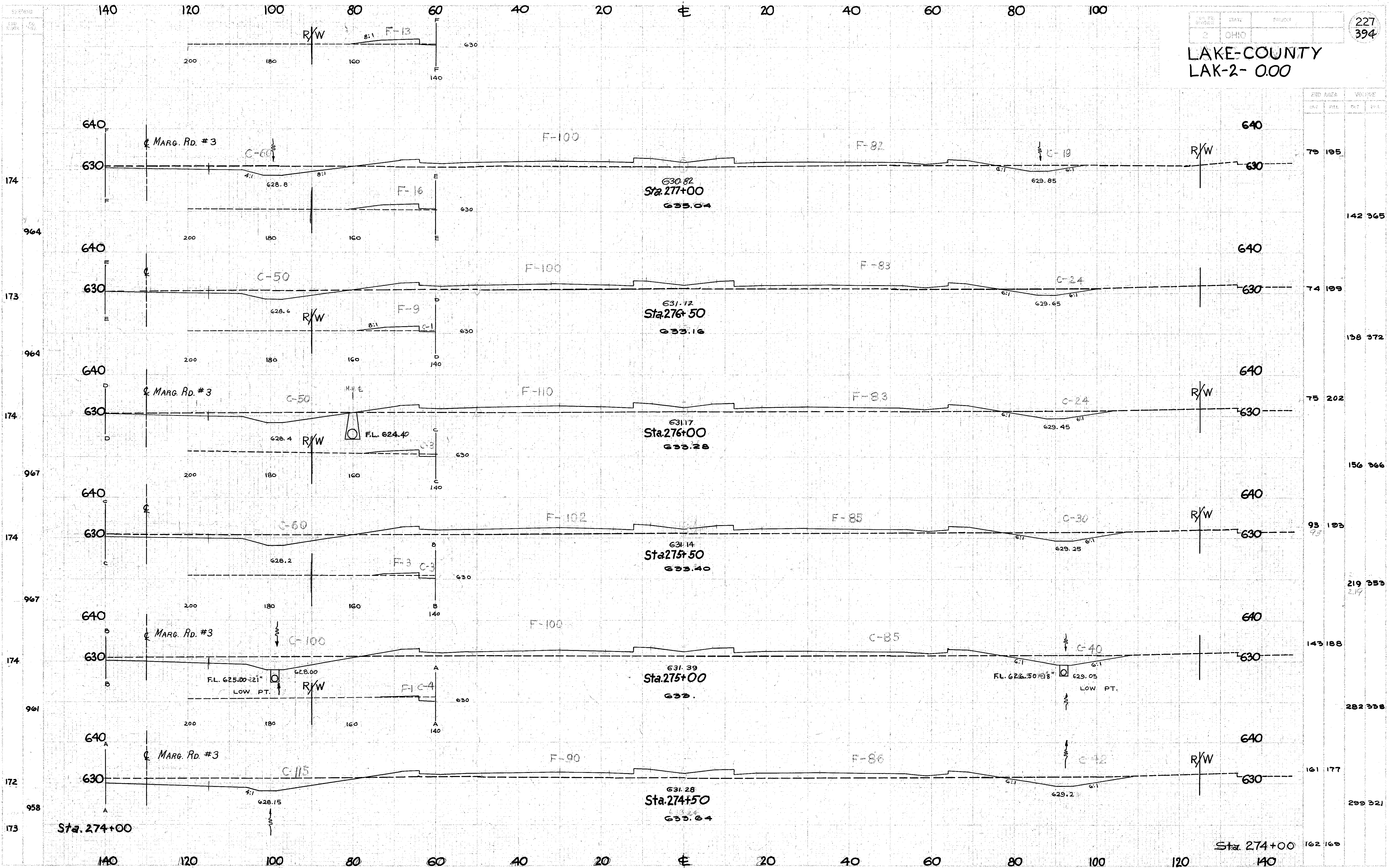
CROSS SECTIONS- STA.274+50 TO STA.277+00
