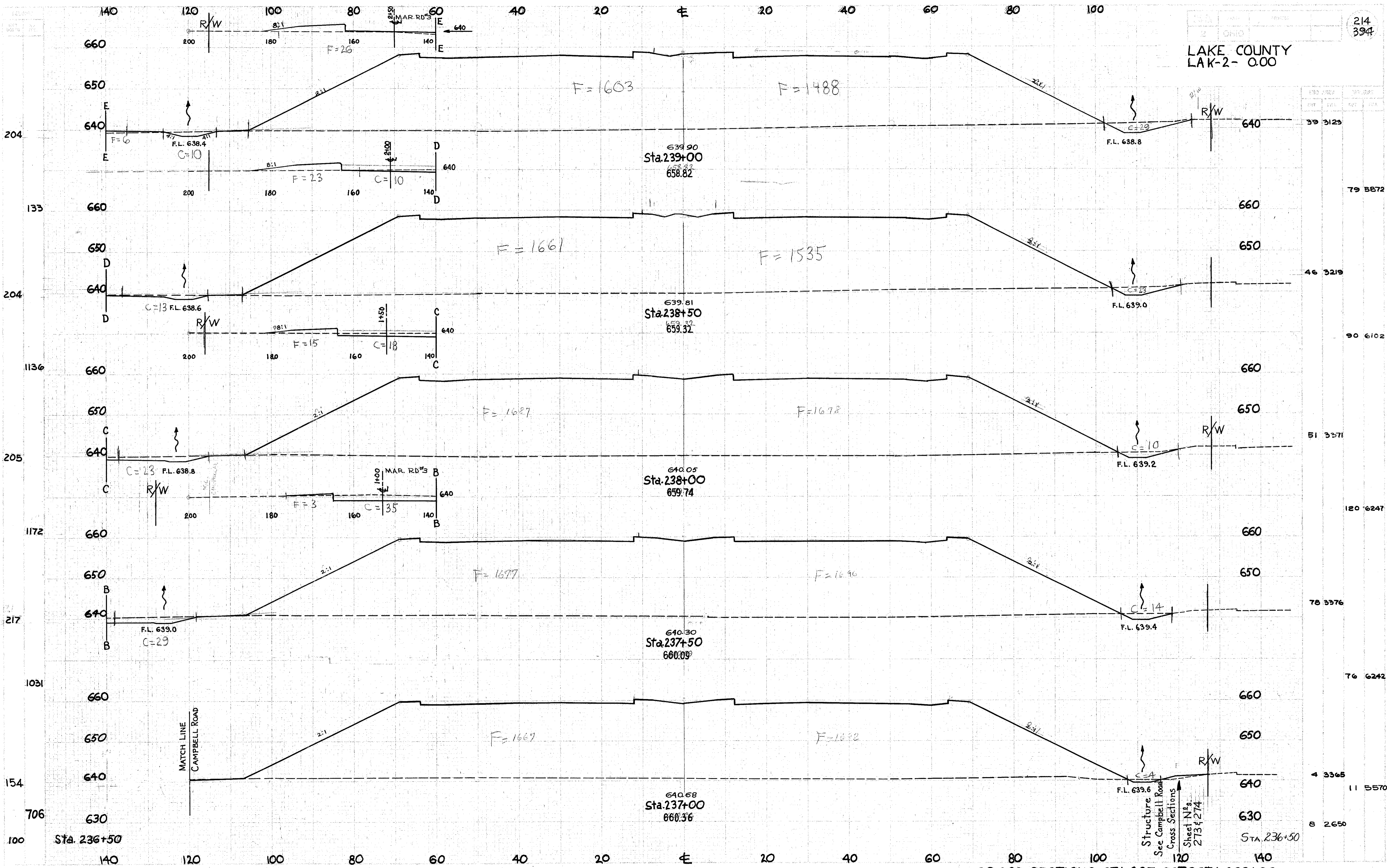
CROSS SECTIONS-STA.237+00 TO STA.239+00
