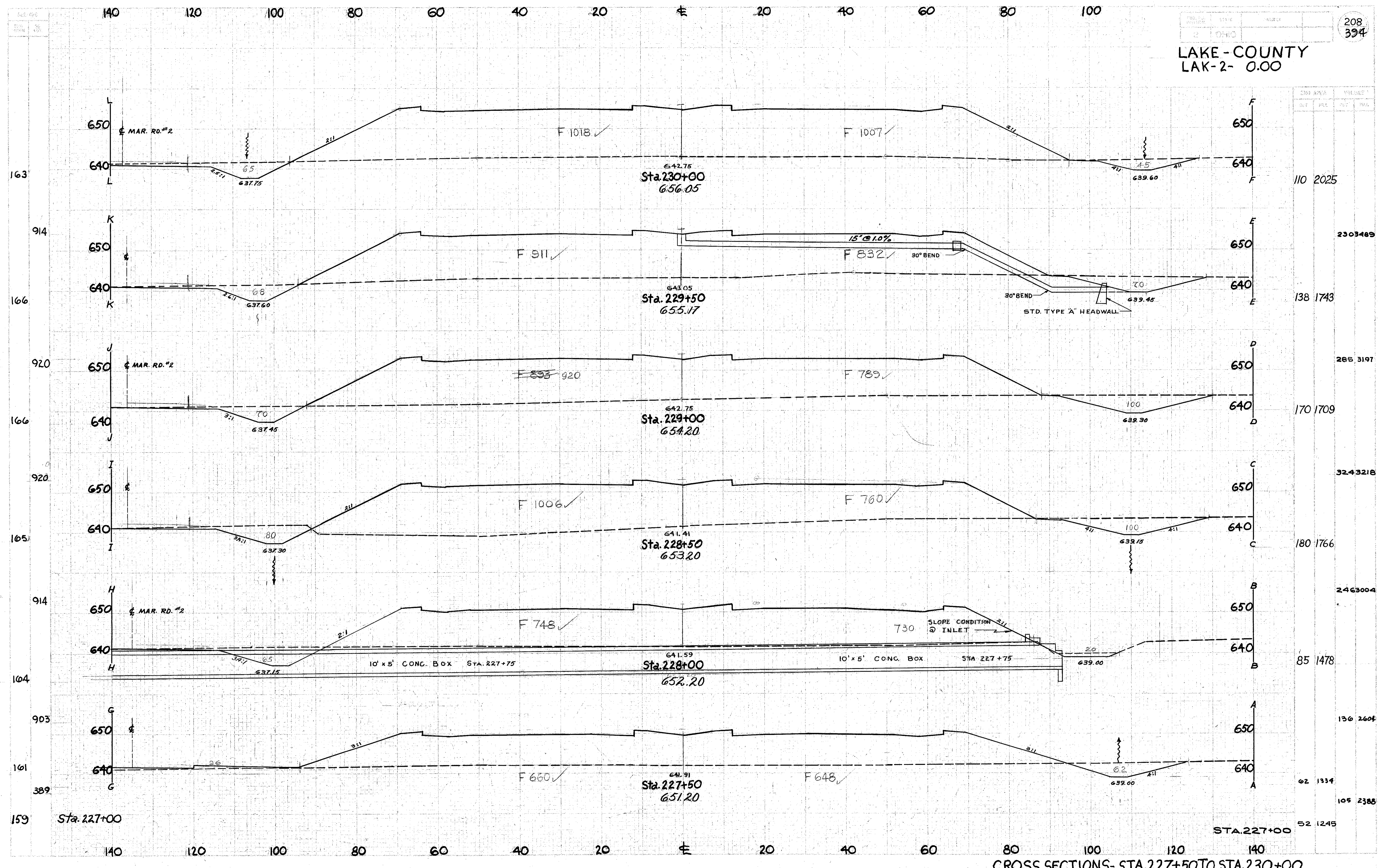
CROSS SECTIONS- STA.227+50 TO STA.230+00
