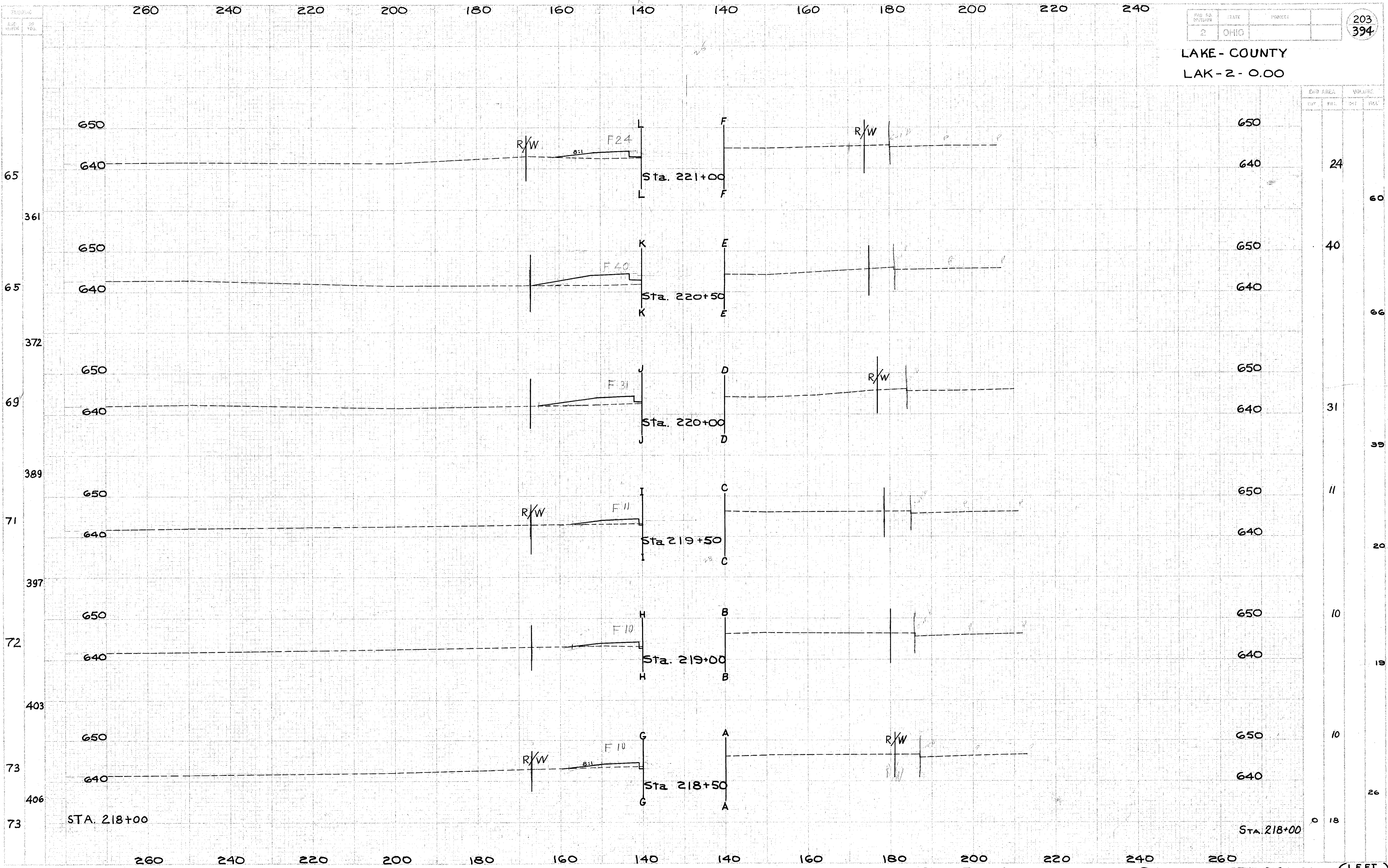
CROSS SECTION EXTENSIONS STA. 218+50 TO STA. 221+00 (LEFT RIGHT)
