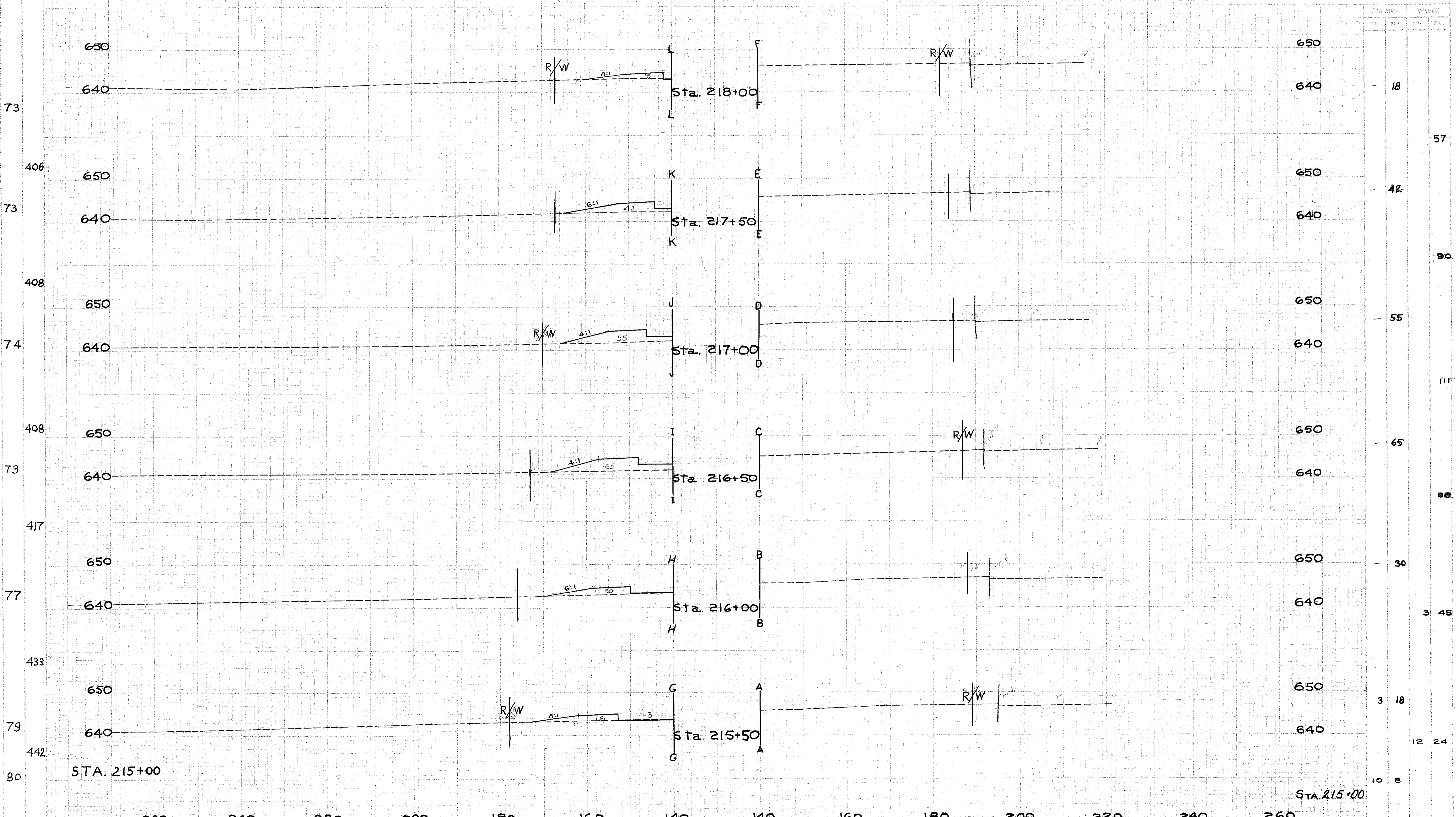
CROSS SECTION EXTENSIONS STA. 215+50 TO STA. 218+00 (LEFT RIGHT)
