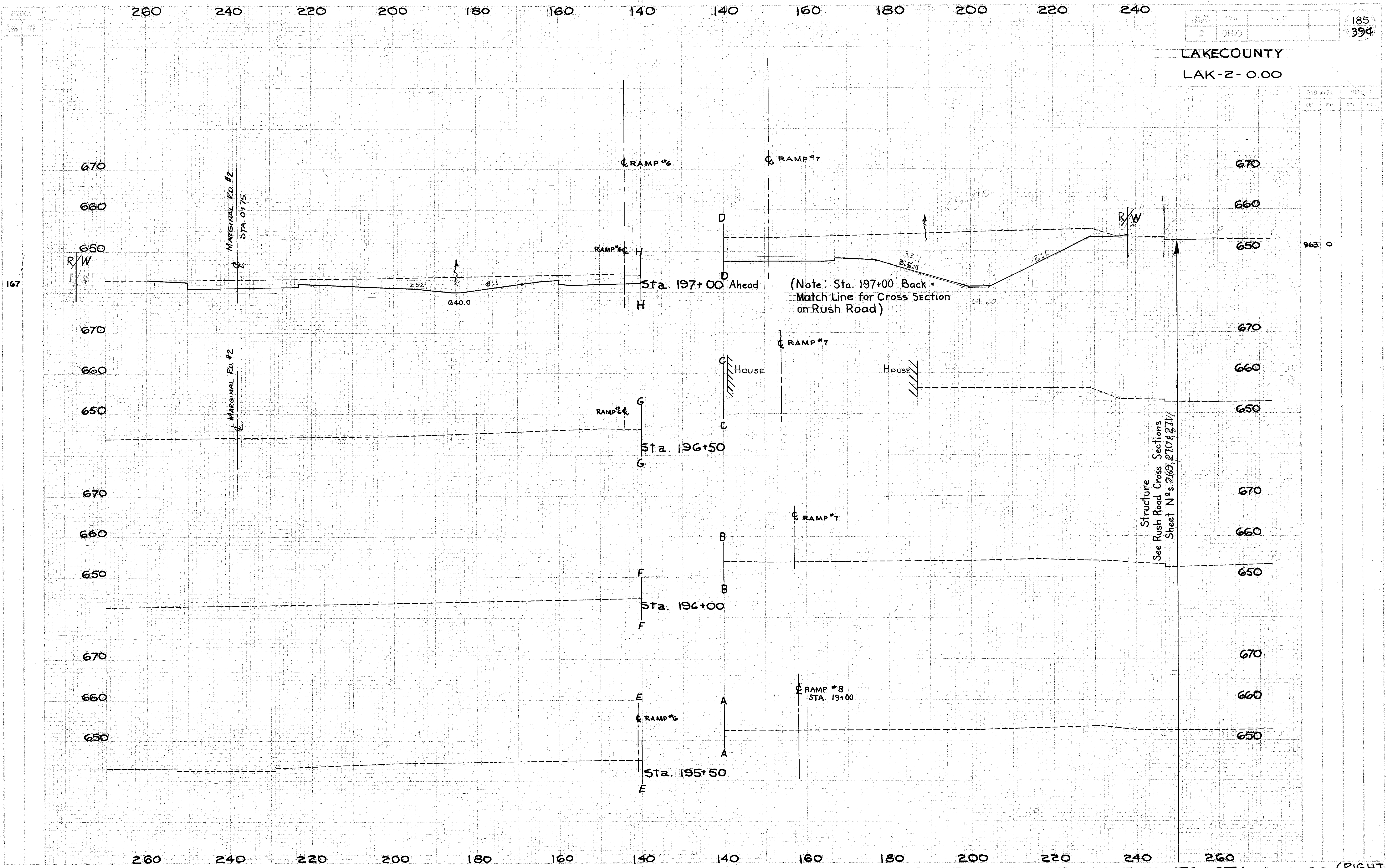
CROSS SECTION EXTENSIONS - STA. 195+50 TO STA. 197+00 (RIGHT & LEFT)
