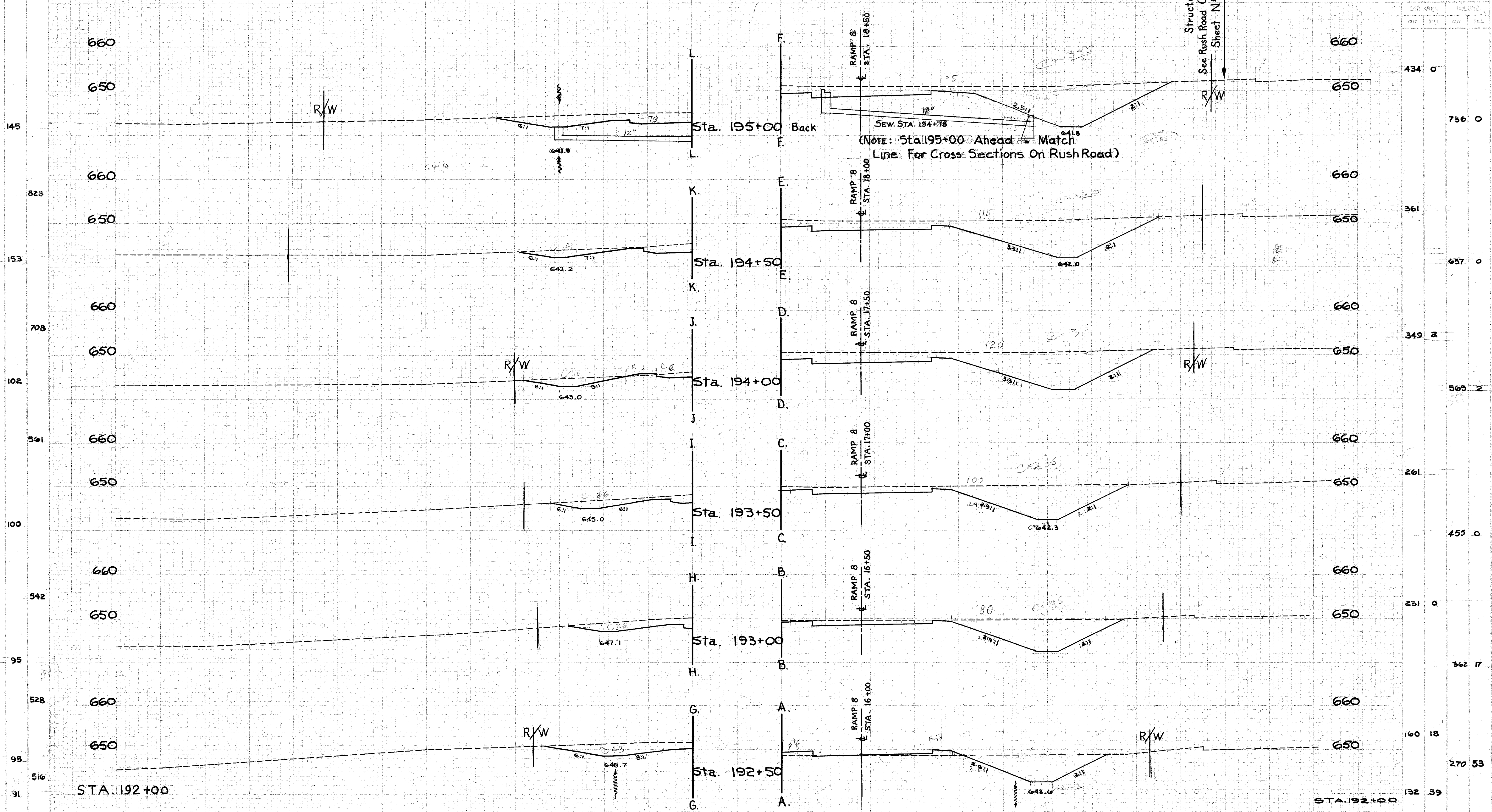
CROSS SECTION EXTENSIONS STA. 192+50 TO STA. 195+00
