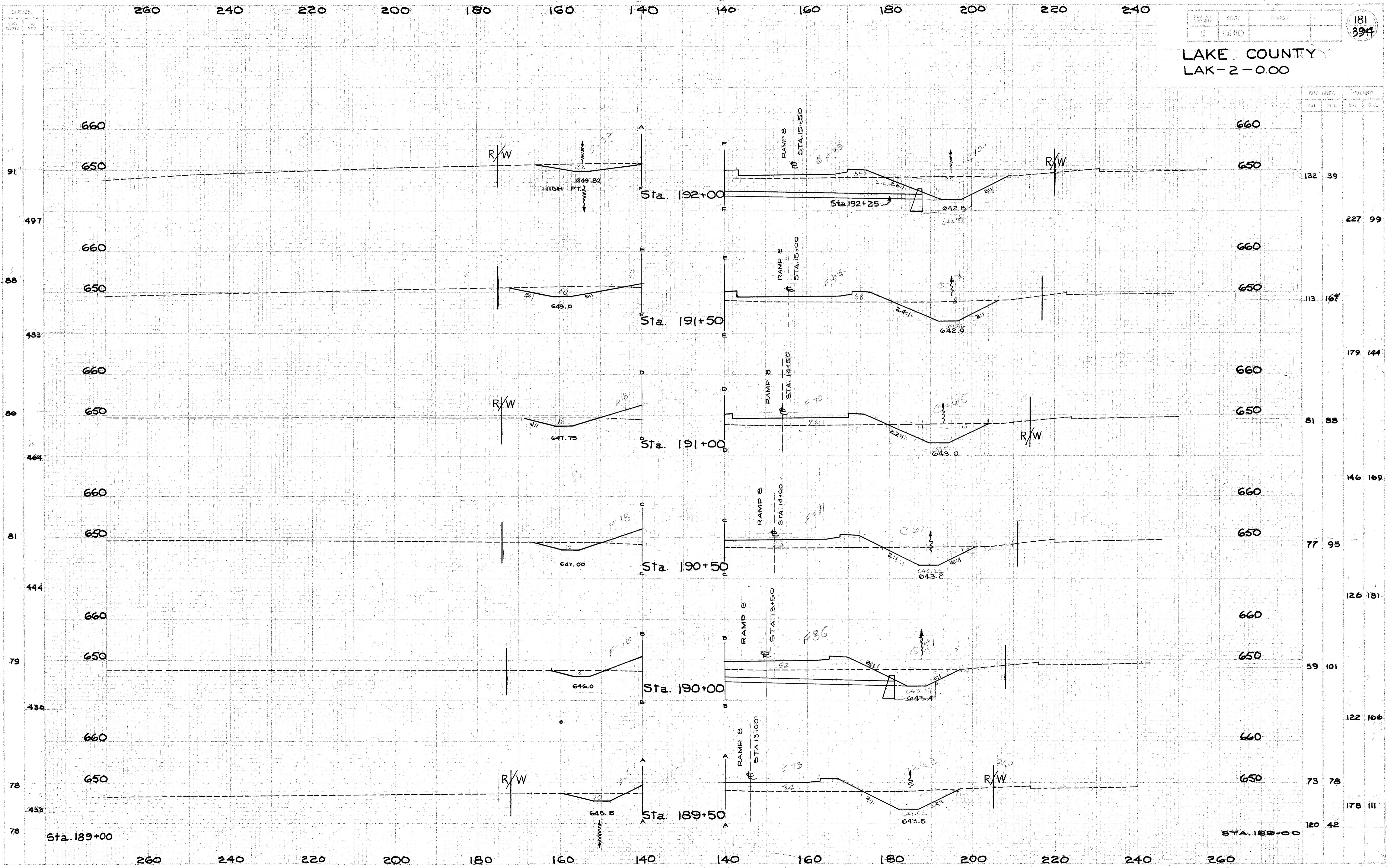
CROSS SECTION EXTENSIONS STA. 189+50 TO STA. 192+00
