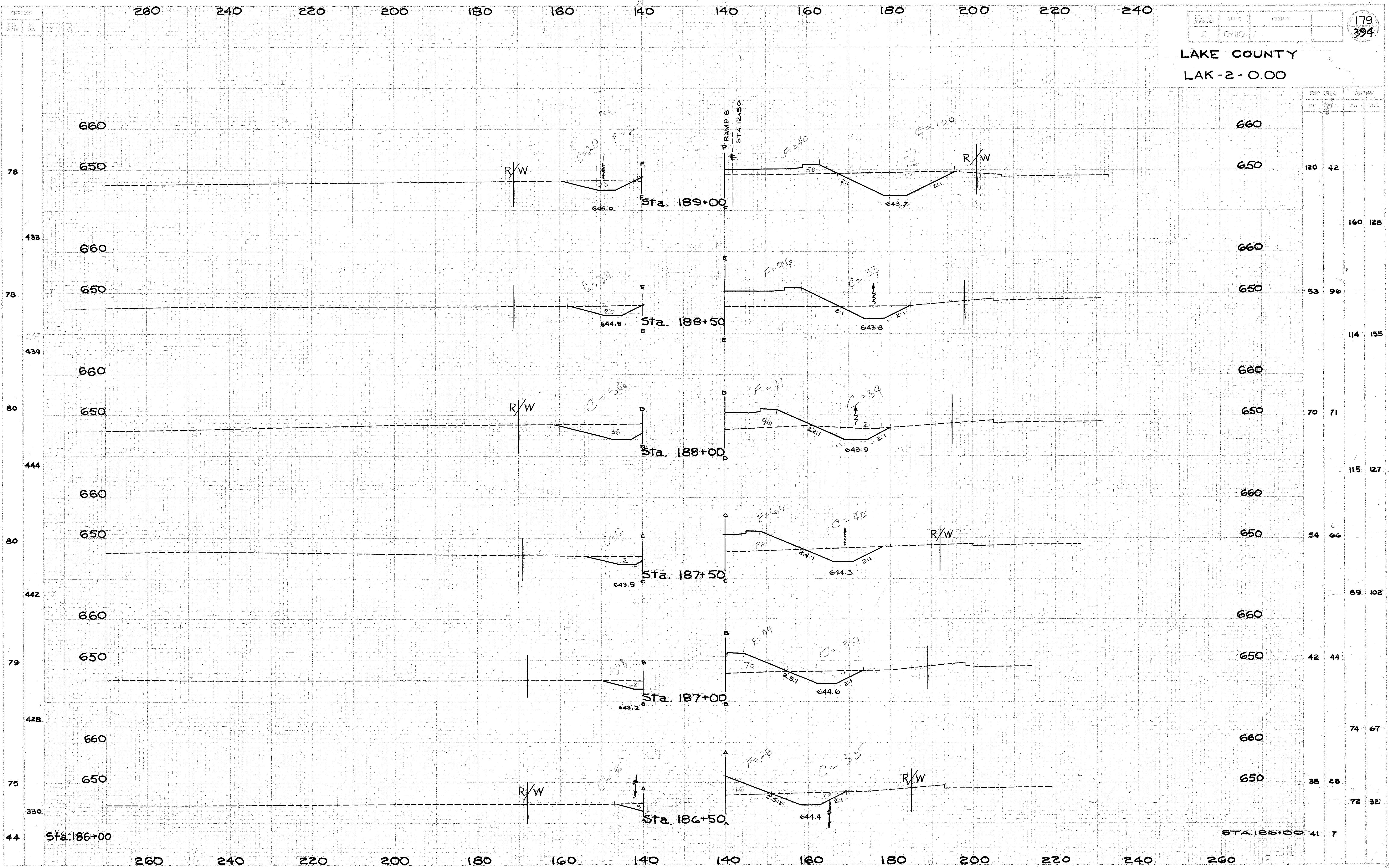
CROSS SECTION EXTENSIONS STA. 186+50 TO STA. 189+00
