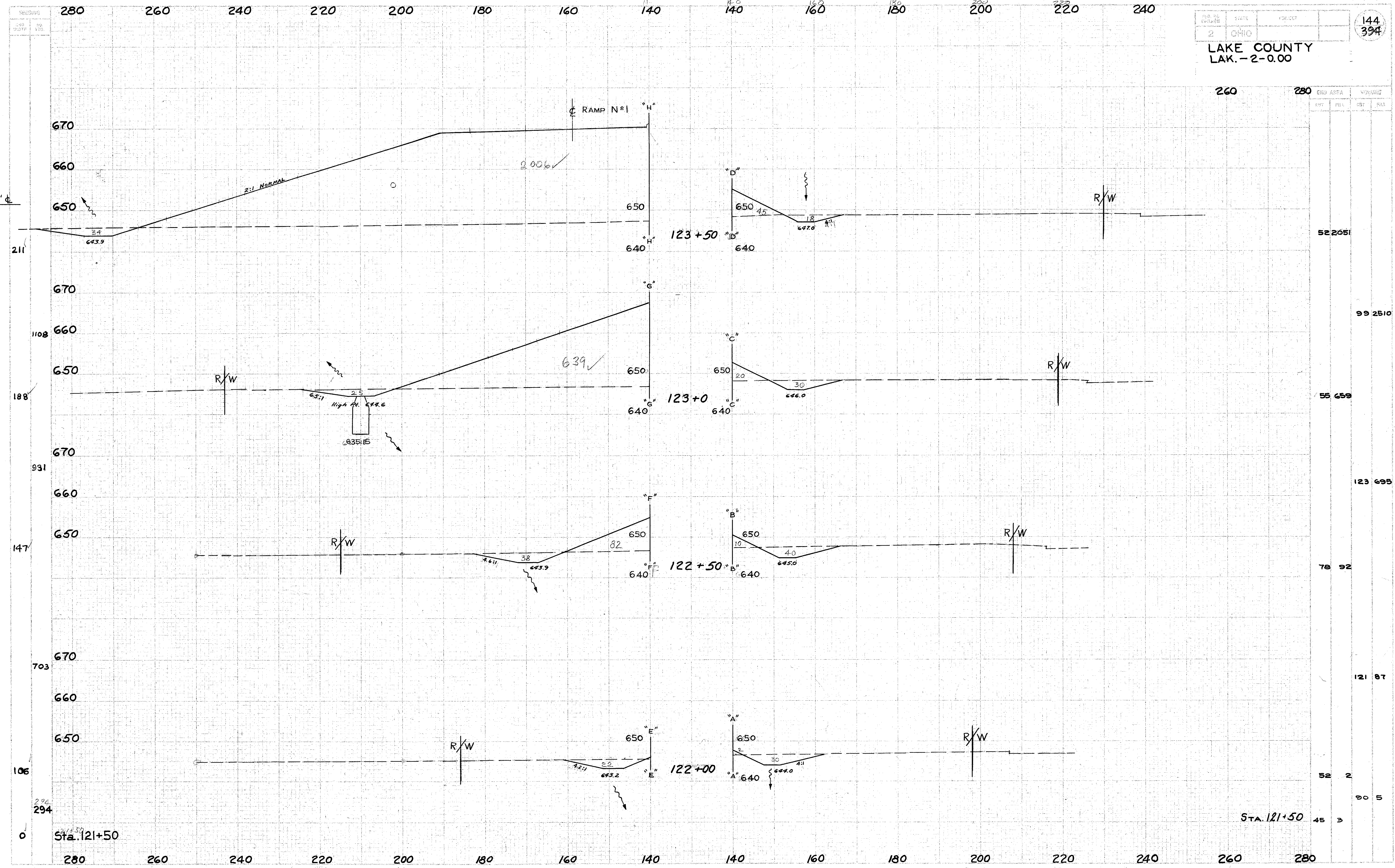
CROSS SECTION EXTENSIONS STA 122+00 to 123+50 RIGHT & LEFT
