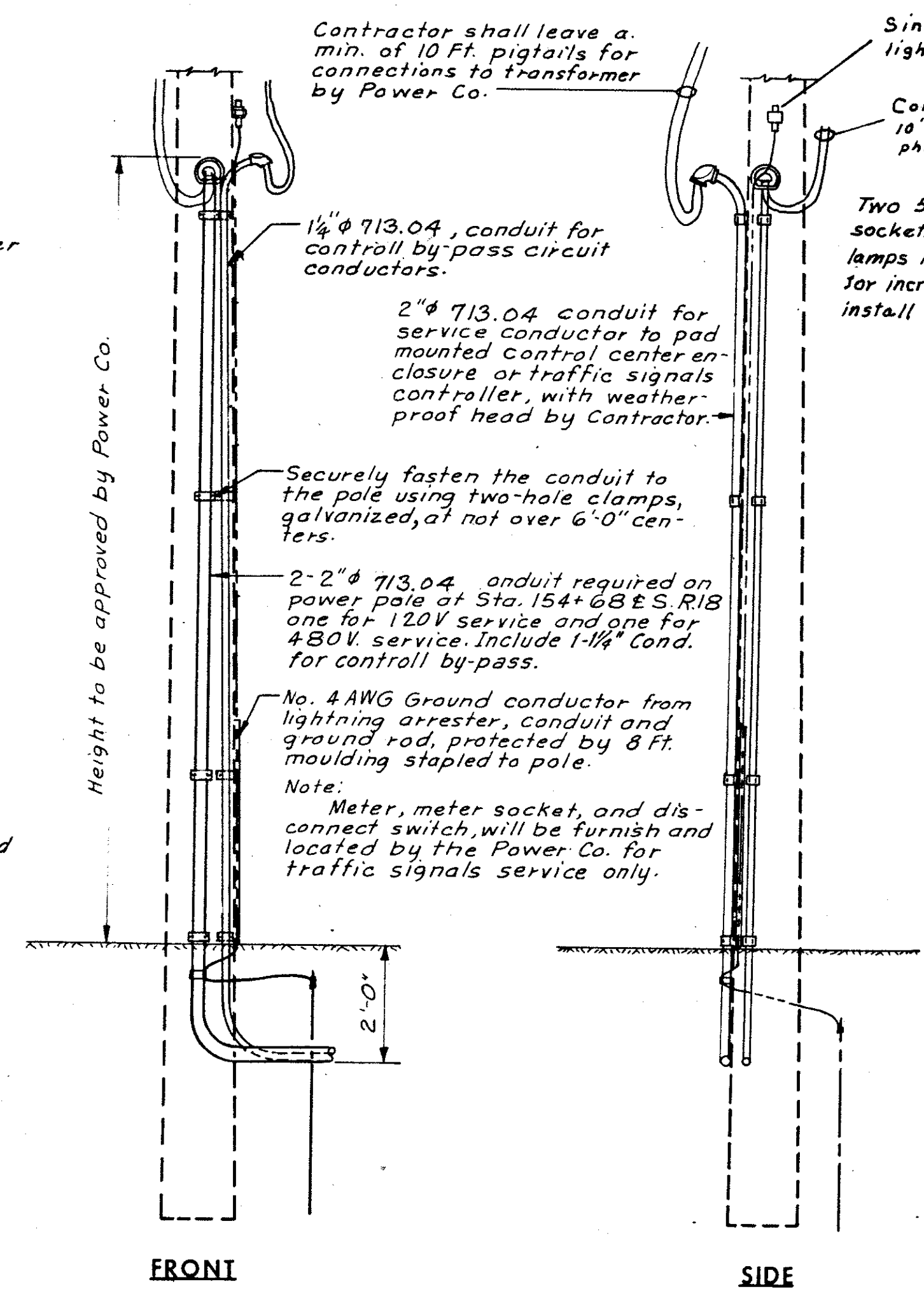
ELECTRICAL SERVICE POWER POLE DETAIL No Scale
