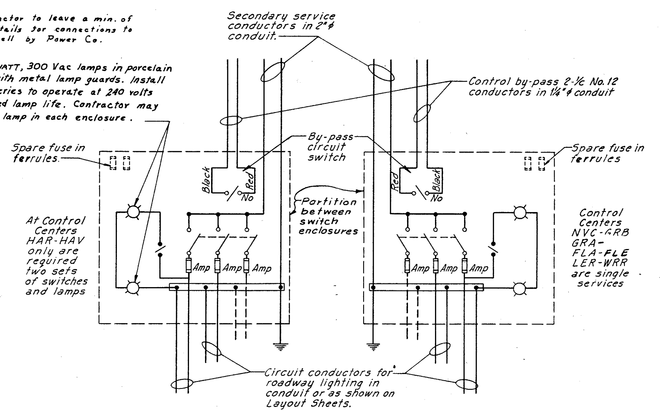
TYPICAL WIRING DIAGRAM IN CONTROL CENTER ENCLOSURE
