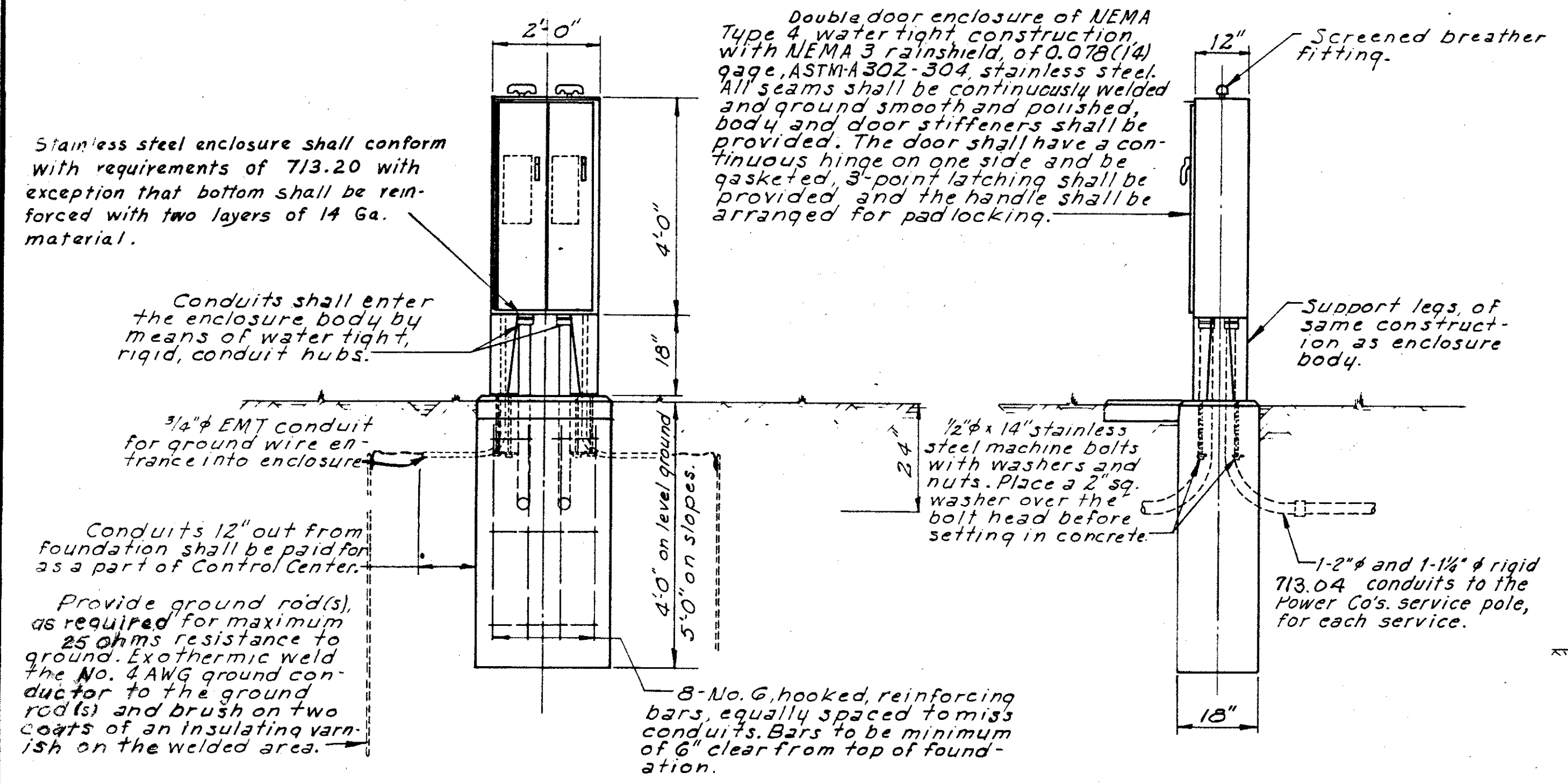
CONTROL CENTER DETAILS Scale: 1/2" = 1'-0"
