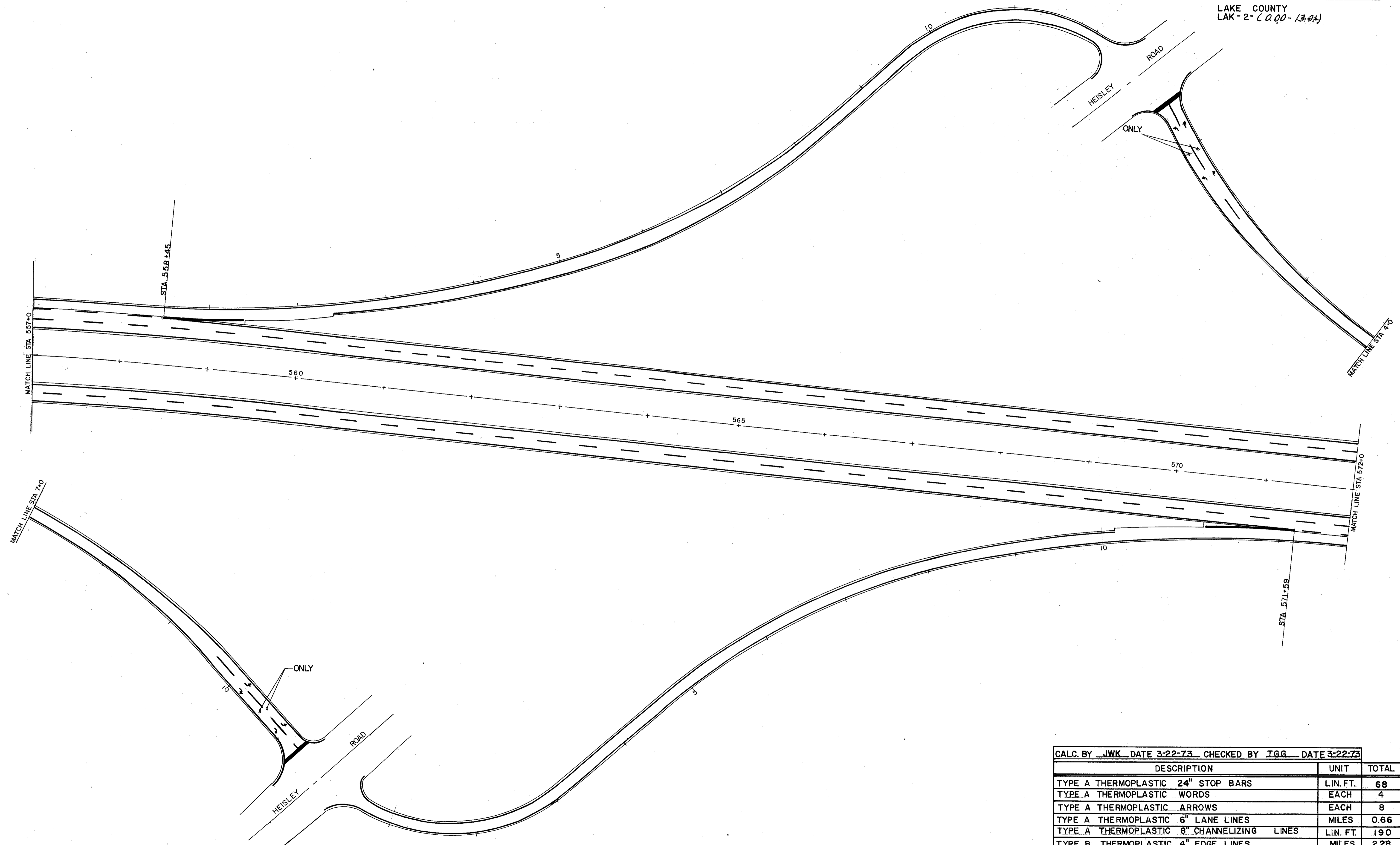
HEISLEY RD. INTERCHANGE PAVEMENT MARKING DETAILS
