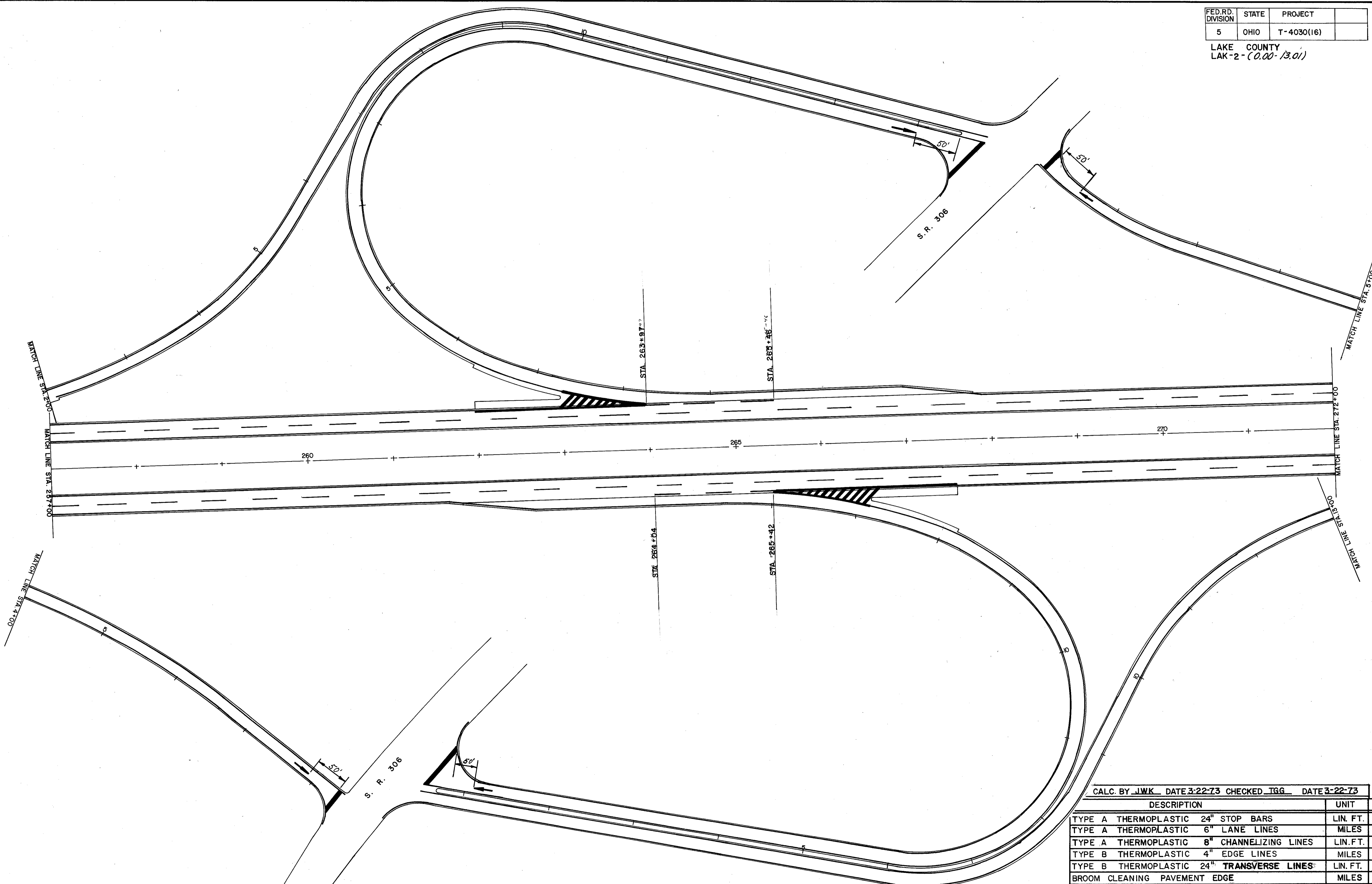
S.R. 306 INTERCHANGE PAVEMENT MARKING DETAILS
