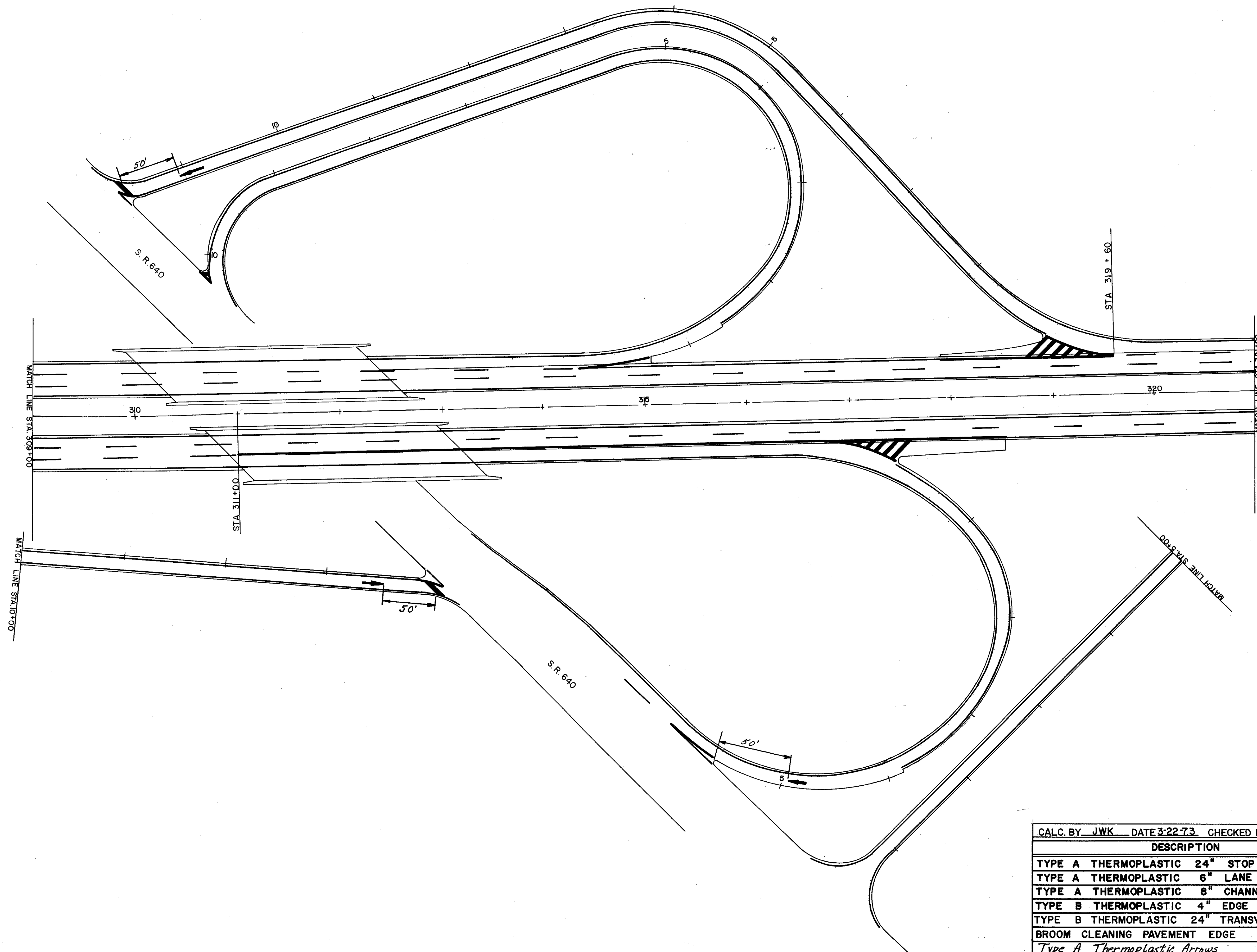
VINE ST. INTERCHANGE PAVEMENT MARKING DETAILS
