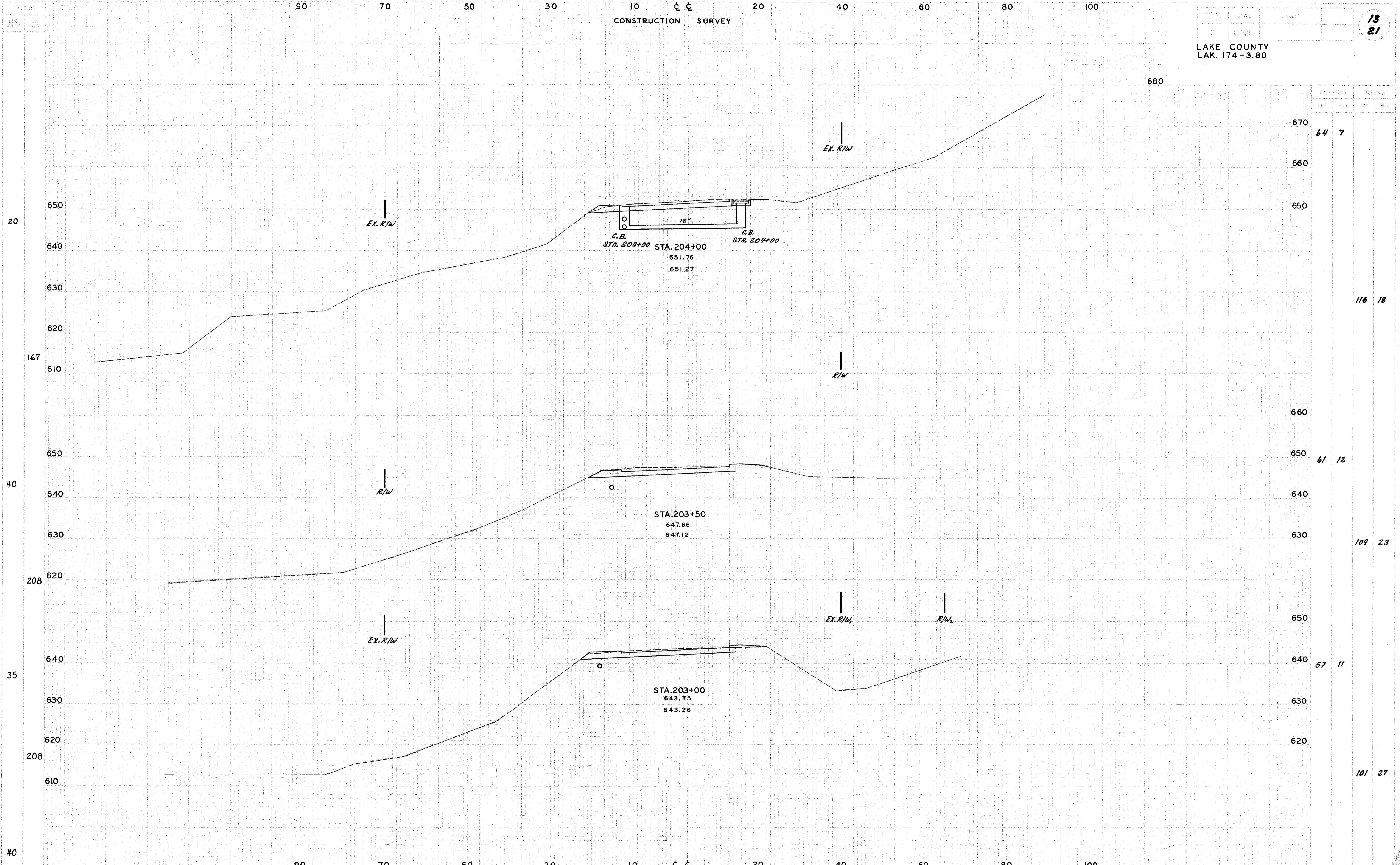
CROSS SECTIONS SR. 174 STA. 203+00 TO 204+00
