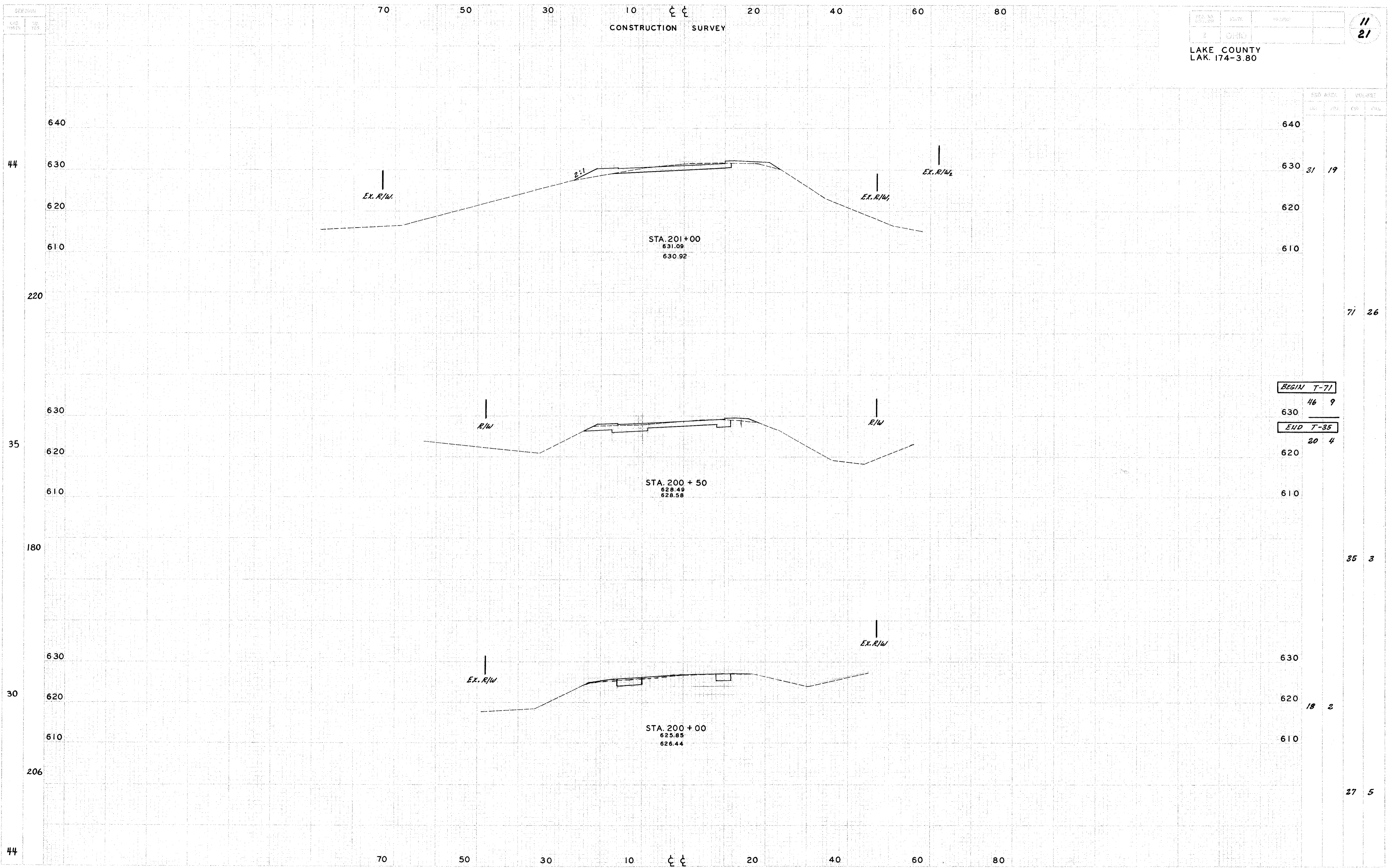
CROSS SECTIONS SR. 174 STA. 200+00 TO 201+00
